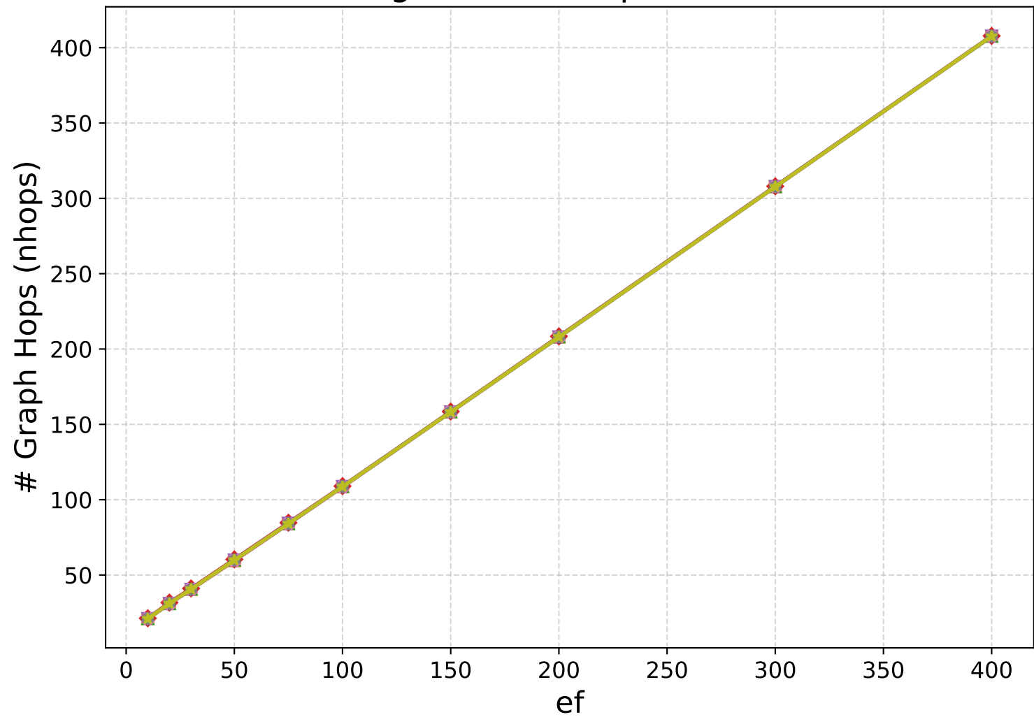
gist1M — nhops vs ef
