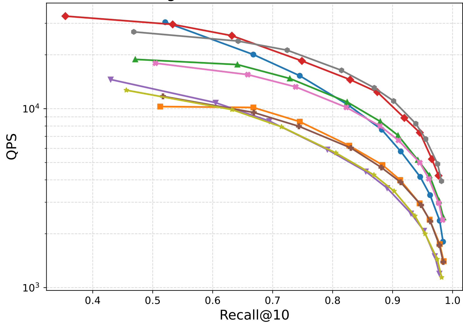
gist1M — QPS vs Recall
