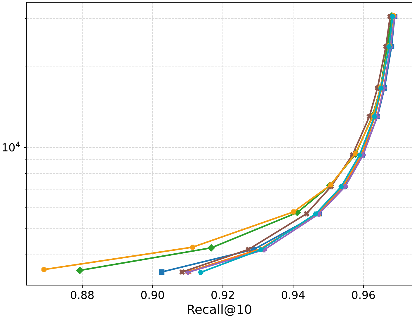
Distance Computations
