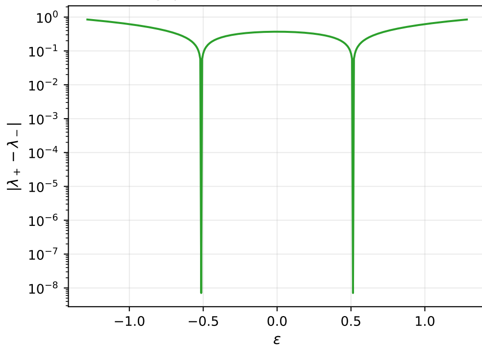
monodromy around EP: 4\pi EP2 YES
