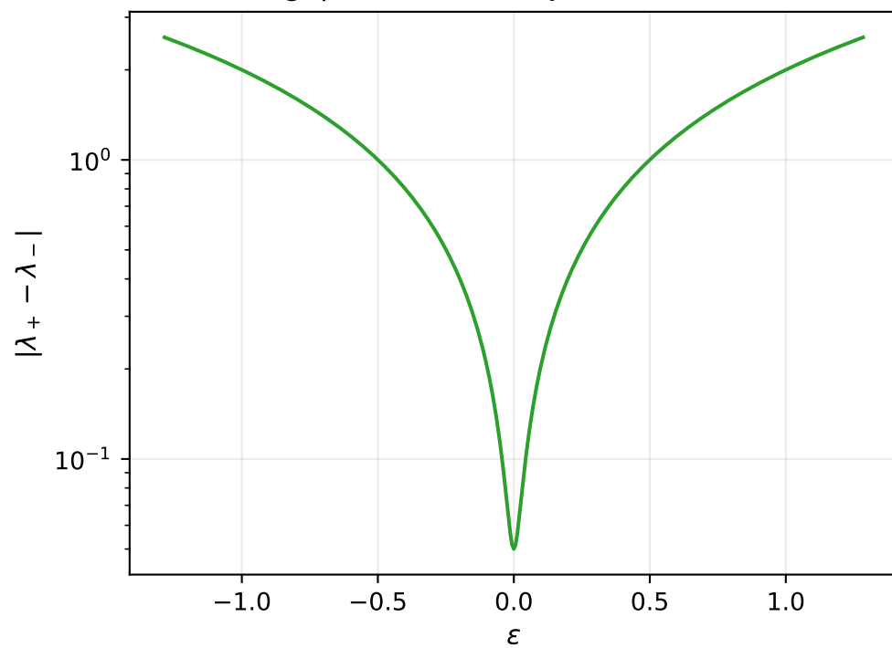
monodromy
