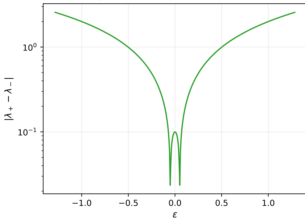
gap ( \text{EP}_2 = 0 with Jordan block)
