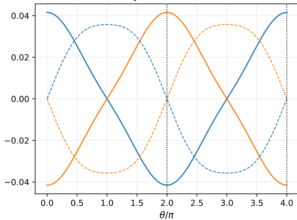
monodromy around EP: 4\pi EP2 YES
