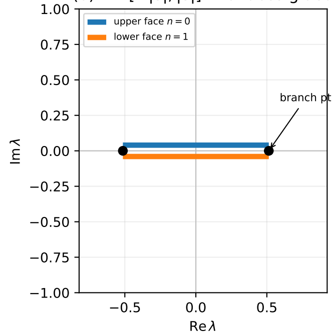
(0) \Gamma = [-|\varepsilon|, |\varepsilon|] two faces glued
