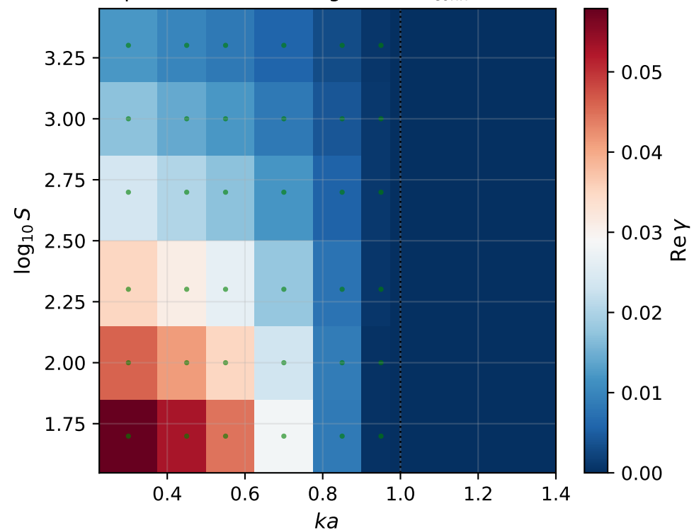
ref tearing mode S = 200, k = 0.55, \gamma = 0.0263
