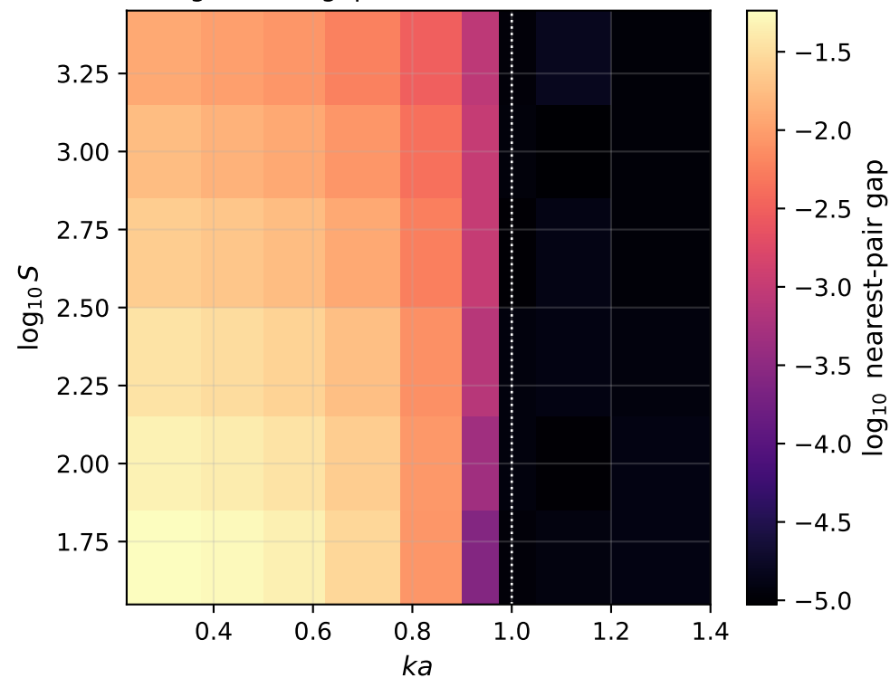
eigenvalue gap (EP candidate = dark)
