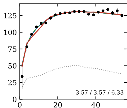
UGC05750
