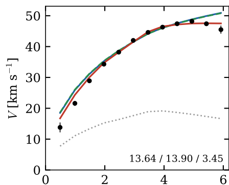
NGC2841
