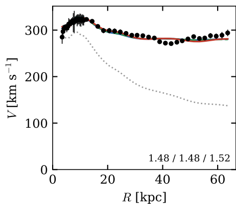
NGC2841
