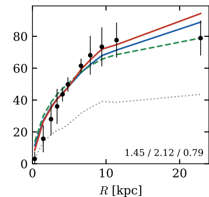
UGC05750
