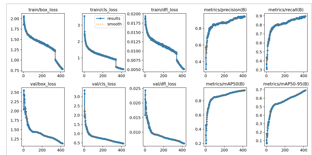
YOLO26s-P2 Training Performance
