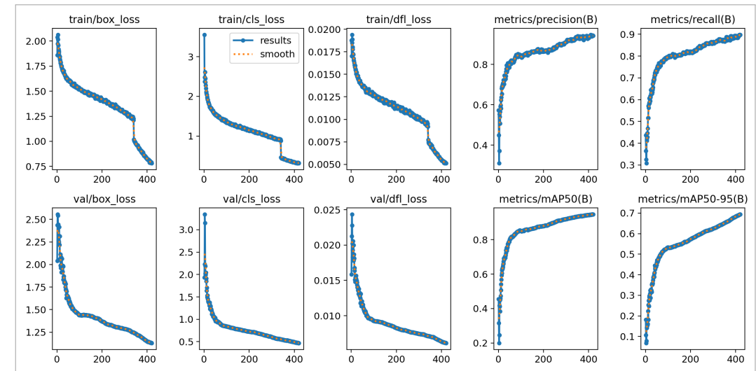
YOLO26s-P2 Training Performance
