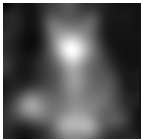
Saliency
