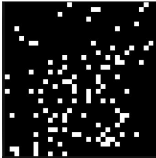
Sampled Tokens
