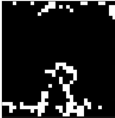
Sampled Tokens
