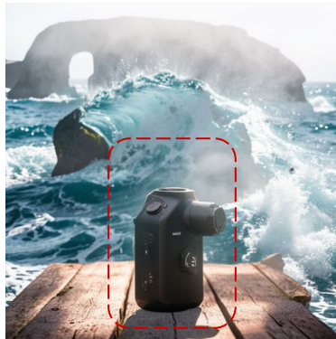
Canny Based
