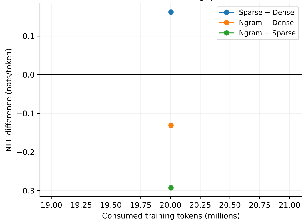
Mixed validation gaps
