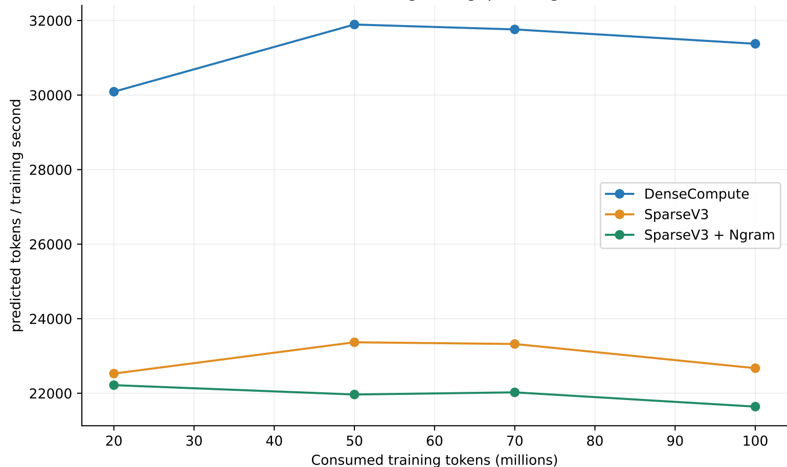
Cumulative training throughput (single run)
