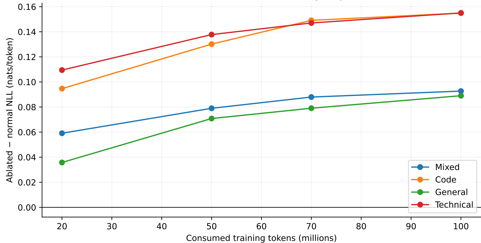
Same-checkpoint Ngram residual-zero ablation Positive delta means memory helps
