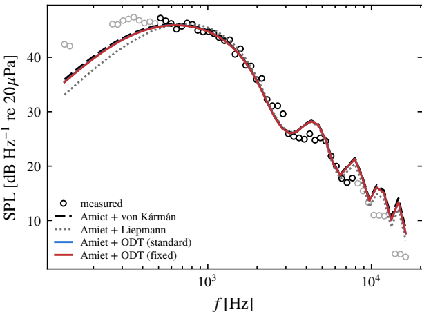
Bampanis 2022 (ECL), flat plate, U=32 m/s
