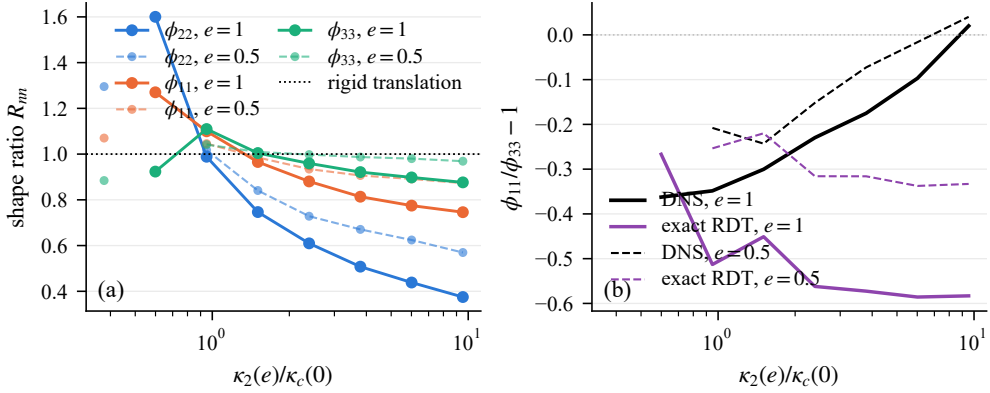
Figure 1. Exact linear theory does not translate the projected spectra rigidly. Left: shape ratio R_{nm}(\kappa_2) of the exactly distorted, line-projected component spectra to a rigid translation, at e = 1 under plane strain (closed-form Cauchy solution, isotropic initial fields, four realisations). Right: the transverse splitting \phi_{11}/\phi_{33} - 1 versus wavenumber in exact linear theory and in the strained-box DNS of § 4.1.
