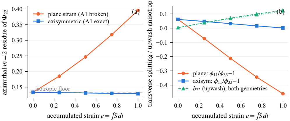
Figure 5. The A1 control experiment at Sk_t/\varepsilon = 16 ( 128^3 , four realisations): axisymmetric contraction (A1 exact by symmetry) against plane strain at matched A_{22} . Left: azimuthal m = 2 residue of \Phi_{22} . Right: transverse splitting and b_{22} .
