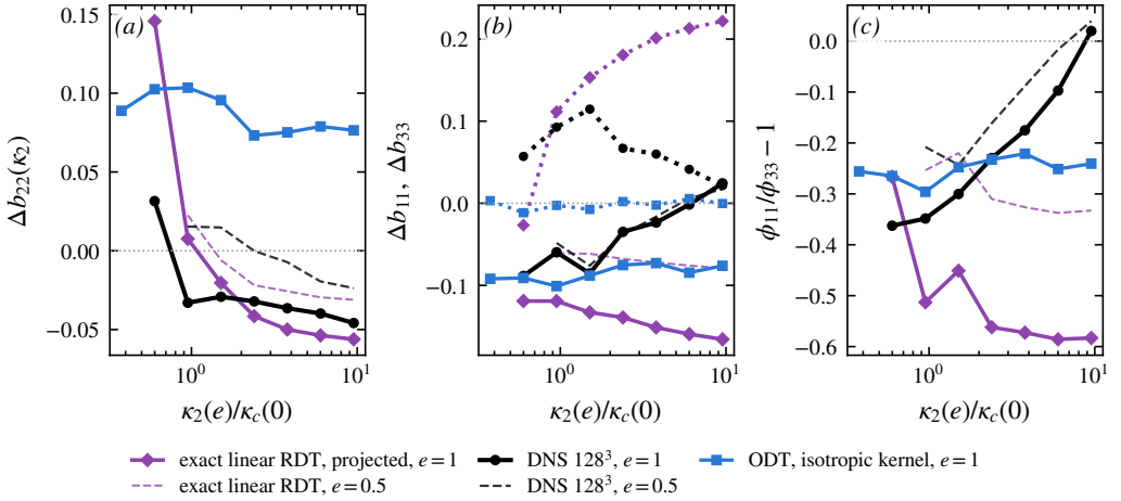
Figure 10. Three-way comparison at Sk_t/\varepsilon = 0.8 : strain-induced anisotropy of the line spectra relative to each system's own unstrained state; SC-ODT (1024 realisations) against exact projected RDT and DNS ( 128^3 , four realisations); e = 1 solid, e = 0.5 dashed.
