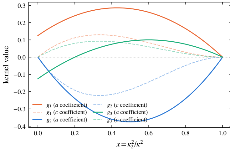
Figure 6. Rapid pressure–strain closure kernels g_1, g_2, g_3 (eqs. (5.7)–(5.9)) against the angular variable x = \kappa_2^2/\kappa^2 . Solid curves: coefficient of the isotropic-like spectral scalar a ; faint dashed curves: coefficient of the anisotropy scalar c . The kernels sum to zero at every x (energy conservation, eq. (5.10)) and vanish at x = 1 . Averaged over an isotropic spectrum they give the ratio +\frac{1}{5} : -\frac{1}{5} : 0 (eq. (5.11)), recovering the isotropisation-of-production form \Pi_{ij}^{(r)} = \frac{4}{5} k_t S_{ij} (Crow 1968) that underlies the moment closure used in § 4.
