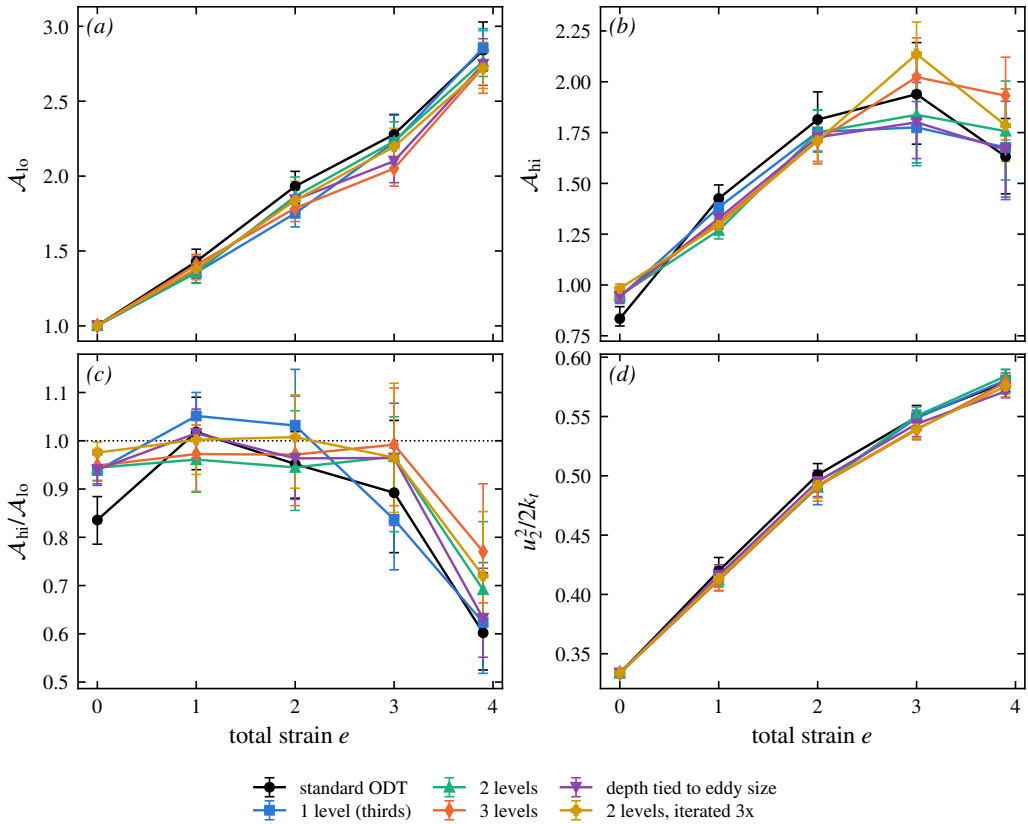
Figure 7. Scale-local relaxation on the transmission diagnostic: (a) energy-containing-band imbalance \mathcal{A}_{lo} , (b) fine-scale-band imbalance \mathcal{A}_{hi} , (c) transmission \mathcal{A}_{hi}/\mathcal{A}_{lo} , (d) upwash energy fraction, against total strain: standard ODT, hierarchical sub-scale kernels at fixed depth (1–3 levels), depth tied to eddy size, and the per-event iterated variant. Medians over 1024 paired-seed realisations, 95% bootstrap intervals.
