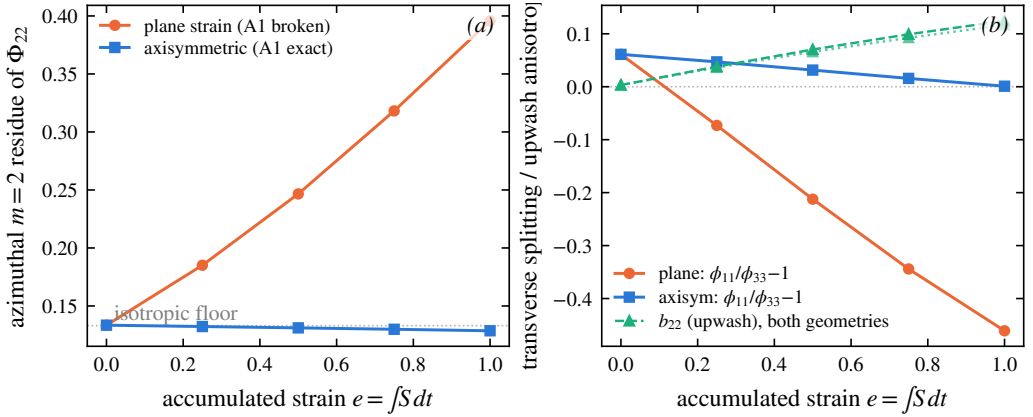
Figure 5. The A1 control experiment at Sk_t/\varepsilon = 16 ( 128^3 , four realisations): axisymmetric contraction (A1 exact by symmetry) against plane strain at matched A_{22} . Left: azimuthal m = 2 residue of \Phi_{22} . Right: transverse splitting and b_{22} .
