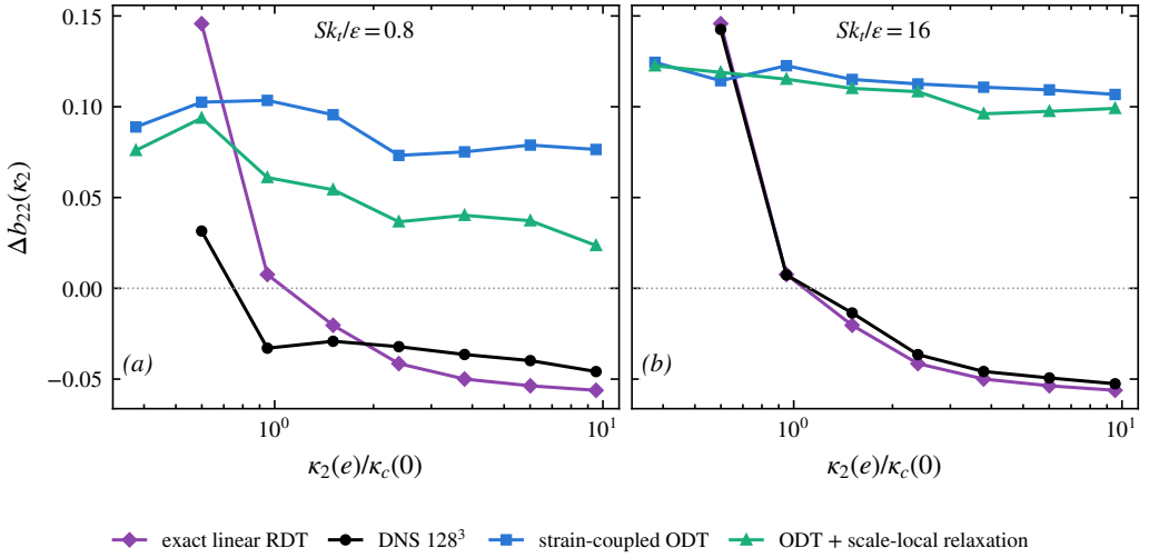
Figure 17. The four-way comparison on the benchmark observable of § 4.2.1: strain-induced upwash anisotropy per wavenumber band at e = 1 , for exact linear RDT, DNS, the strain-coupled model, and the model with adaptive-depth scale-local relaxation, at (a) Sk_t/\varepsilon = 0.8 and (b) 16 (ODT: 1024 realisations per case, same binary and precursor protocol; DNS and companions as in § 4.2). At rapid strain the DNS realises the exact-RDT allocation; scale-local relaxation moves the model towards the DNS at moderate rapidity and only marginally at rapid strain.
