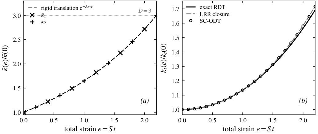
Figure S1. Rapid-distortion limit (eddy events suppressed, inviscid) against the analytic reference of ? used by ?. (a) Component spectral-centroid migration: the streamwise ( \times ) and upwash ( + ) centroids both follow the rigid-translation law and coincide throughout (the markers are interleaved so the two coincident series stay legible), reaching the deformation ratio D = 3 at the end of the straining phase. (b) Kinetic-energy amplification: the solver follows the closure trajectory, within 2% of the exact rapid-distortion value at e = 2.20 .
