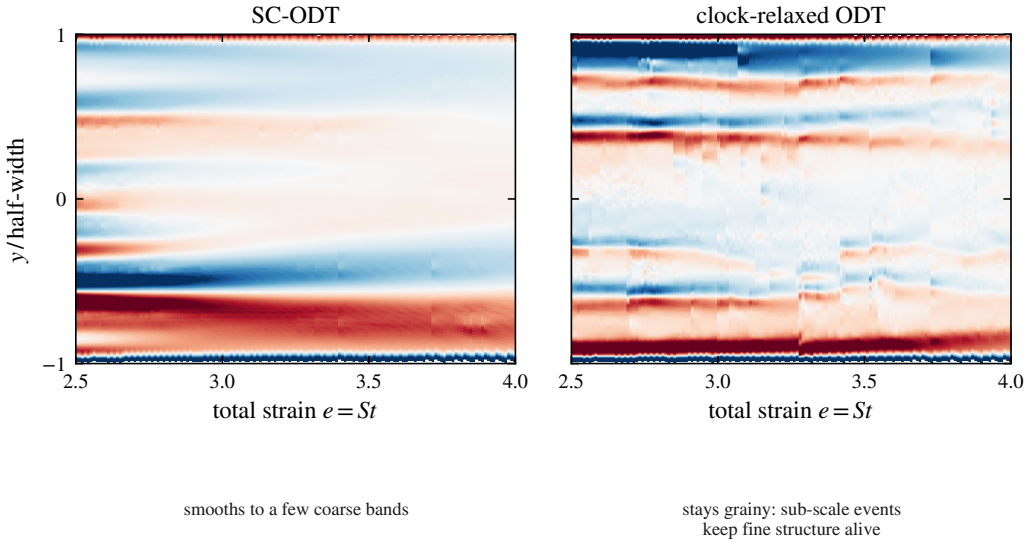
Figure S7. Small-scale (high-pass) upwash structure of a single ODT line in the high-strain window, e = 2.5 – 4 , in the stretched coordinate y/\text{half-width} : SC-ODT (left) against clock-relaxed ODT (right); blue positive, red negative, colour intensity the magnitude. SC-ODT smooths to a few coarse bands; the clock-relaxed line stays grainy, its sub-scale relaxation events sustaining fine-scale structure (the vertical striations are individual events). Amplitudes are normalised and the two are different realisations, so the contrast is the clock's structural signature, not a pointwise difference.
