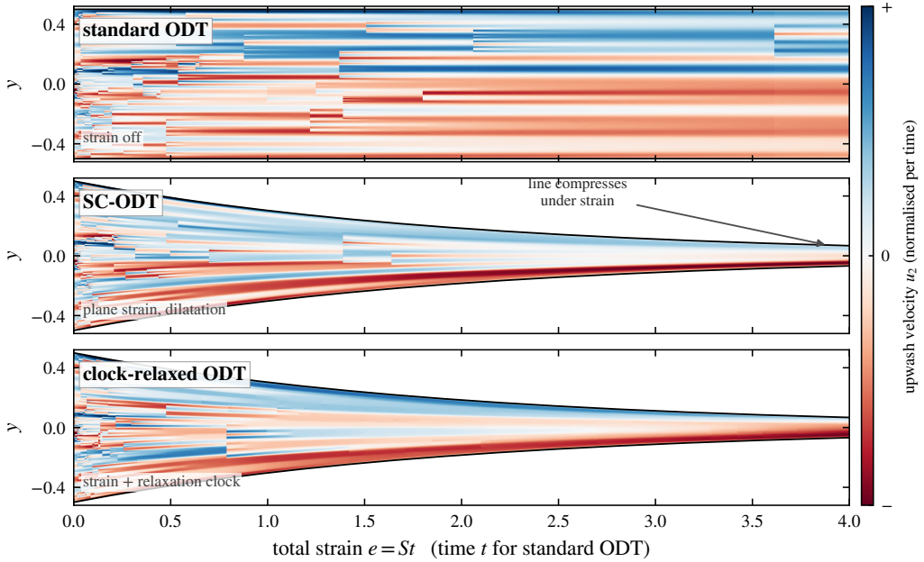
Figure S6. Space–time evolution of the ODT line, upwash velocity u_2 (normalised at each instant; blue positive, red negative, colour intensity the magnitude), for standard ODT, SC-ODT and clock-relaxed ODT, advanced from matched initial fields. Time runs left to right as the total strain e = St (elapsed time for the unstrained standard-ODT case); the black envelope is the physical line half-width. Standard ODT keeps its full width; SC-ODT and clock-relaxed ODT compress under the plane strain, the clock-relaxed line retaining finer structure at high strain.
