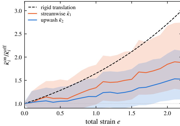
Figure 11. Full model (eddies and viscosity active; ensembles over 128 realisations at \nu = 10^{-5} ): strain-induced migration of the streamwise and upwash component centroids, each as the ratio of the strained ensemble to the matched no-strain baseline, against the rigid-translation law (dashed). The components diverge under strain—the upwash held back most—reproducing the qualitative departure-from-RDT mechanism of Chen et al. (2006) . The comparison is qualitative; see text.
