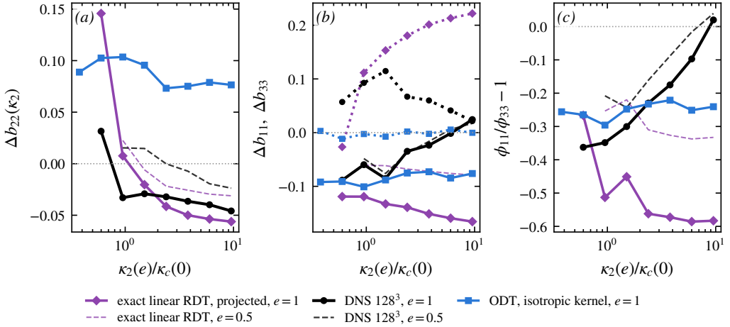
Figure 12. Three-way comparison at Sk_t/\varepsilon = 0.8 : strain-induced anisotropy of the line spectra relative to each system's own unstrained state; strain-coupled ODT (1024 realisations) against exact projected RDT and DNS ( 128^3 , four realisations); e = 1 solid, e = 0.5 dashed.
