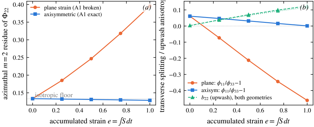
Figure 14. The A1 control experiment at Sk_t/\varepsilon = 16 ( 128^3 , four realisations): axisymmetric contraction (A1 exact by symmetry) against plane strain at matched A_{22} . Left: azimuthal m = 2 residue of \Phi_{22} . Right: transverse splitting and b_{22} .
