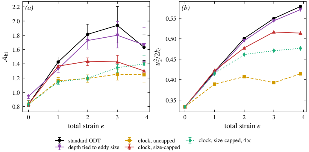
Figure 17. The independent relaxation clock against the eddy-locked family. (a) Fine-scale-band imbalance \mathcal{A}_{hi} against total strain: the eddy-locked variants fade beyond e \approx 3 ; the clock holds at every strain. (b) The price: upwash energy fraction—the uncapped clock suppresses the physical one-point anisotropy, the size cap restores it. Medians over 1024 paired-seed realisations; the clock rate is matched to the baseline eddy rate.
