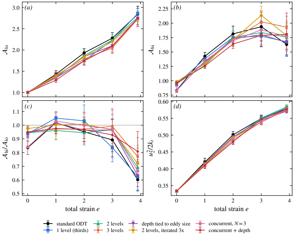
Figure 16. Scale-local relaxation on the transmission diagnostic: (a) energy-containing-band imbalance \mathcal{A}_{lo} , (b) fine-scale-band imbalance \mathcal{A}_{hi} , (c) transmission \mathcal{A}_{hi}/\mathcal{A}_{lo} , (d) upwash energy fraction, against total strain: standard ODT, hierarchical sub-scale kernels at fixed depth (1–3 levels), depth tied to eddy size, the per-event iterated variant, concurrent relaxation ( N = 3 randomly placed same-size intervals per event), and the stacked variant (concurrent intervals each running the adaptive hierarchy). Medians over 1024 paired-seed realisations, 95% bootstrap intervals.
