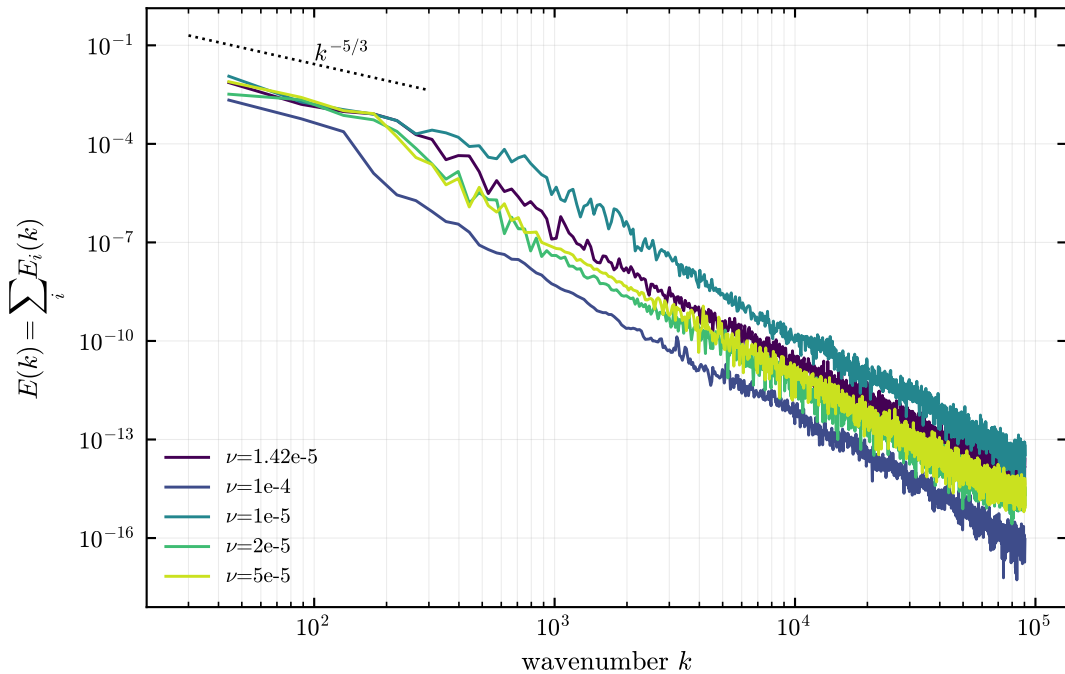
Final-strain spectrum vs \nu (cascade depth)
