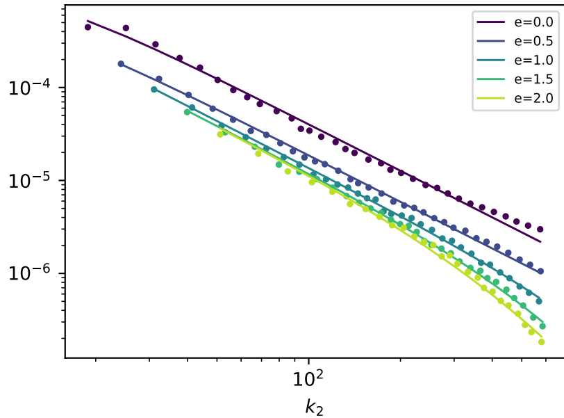
E_2(k_2) (upwash), median + fit
