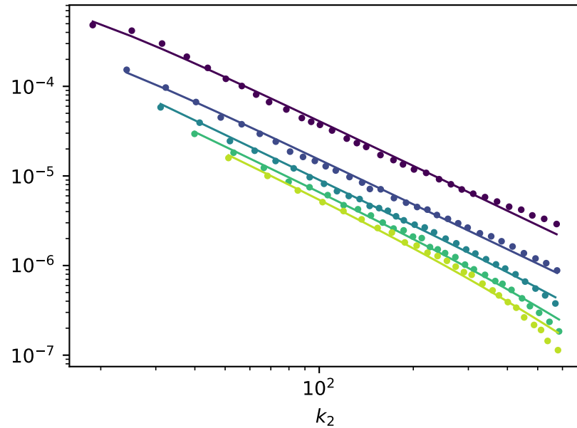
E_{\perp}(k_2) , median + fit
