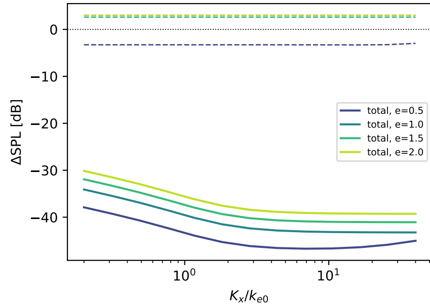
Gate B (solid: vs e=0 fit; dashed: shape-only)
