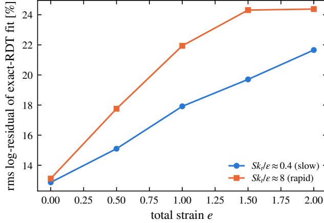
Figure 14. Scale-resolved distance between the strained ODT line spectra and exact linear theory: rms log-residual of the two-parameter exact-RDT-distorted von Kármán fit, against total strain, for slow and rapid onset strain-rate parameters (medians over 1024 realisations; identical precursor state at e = 0 ).
