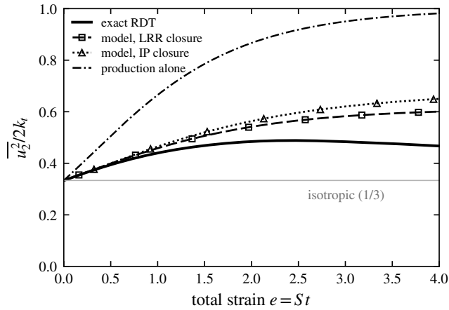
Figure 3. Upwash energy fraction under plane strain for initially isotropic turbulence: exact rapid-distortion theory, SC-ODT with the LRR and IP closures, and production alone ( B_{ij} = 0 ). Production without the rapid term overstates the onset amplification rate by \frac{5}{2} and forces almost all the energy into the upwash component; the rapid term restores the physical, bounded amplification.
