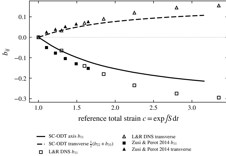
Figure 6. Reynolds-stress anisotropy under axisymmetric contraction: SC-ODT (lines; ensemble mean over 1000 realisations) against the DNS of Lee & Reynolds (1985) (open markers) and the independent DNS of Zusi & Perot (2014) (filled markers, their highest rate, over c \leq 1.65 ). Solid/□: the compressed axial component b_{11} ; dashed/△: the transverse component \frac{1}{2}(b_{22} + b_{33}) . The model tracks the sign and monotonic growth of both, and the two DNS agree where they overlap; the magnitude is under-predicted at large strain by the closure gap common to the second-moment family (§ 3.2), not by the line.
