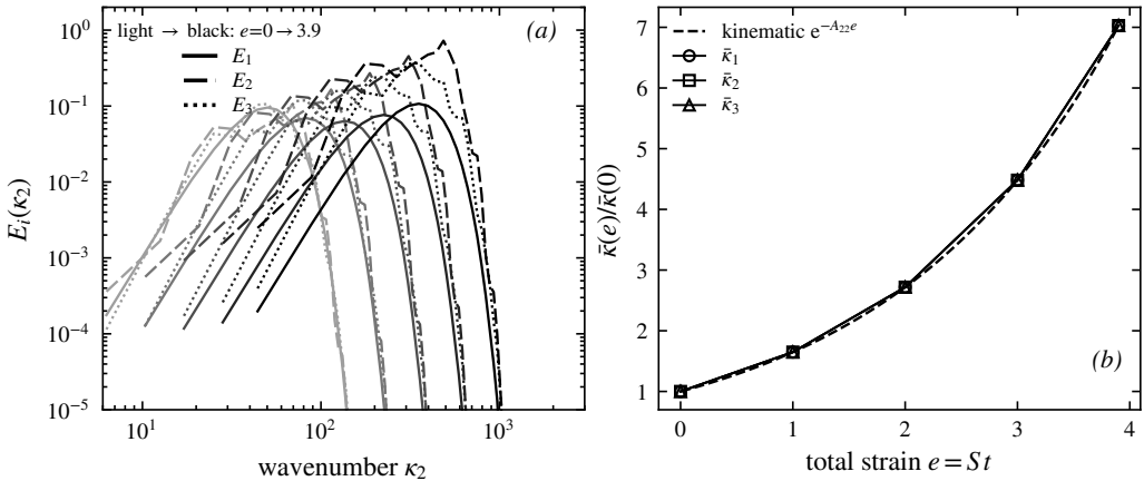
Figure 9. Compression without cascade (eddy events suppressed, inviscid). (a) Component line spectra E_i(\kappa_2) at total strains e = 0, 1, 2, 3, 3.9 (lighter to darker); the spectra translate to higher wavenumber without changing shape. (b) Spectral-centroid migration \bar{\kappa}(e)/\bar{\kappa}(0) for each component (symbols) against the kinematic prediction e^{-A_{22}e} (dashed). The centroid follows the prediction and the three components coincide, confirming purely geometric compression of the line.
