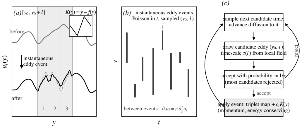
Figure 1. The model at a glance. (a) An eddy event: on the sampled interval [y_0, y_0 + l] the triplet map compresses each profile threefold, inserts three images (the central one reversed, images numbered), and the kernel addition c_i K(y) (inset; dotted: the mapped profile before it) redistributes kinetic energy among the components at conserved per-component momentum and total energy; the exterior is untouched. (b) The two interleaved mechanisms in the space–time plane: eddy events are instantaneous (vertical bars: position and size as sampled), arriving as a Poisson sequence whose rate density is set by the instantaneous flow state, while between events the fields advance by deterministic diffusion and, from § 2.3 onward, the continuous mean-strain forcing. (c) The corresponding advancement cycle of the implementation.
