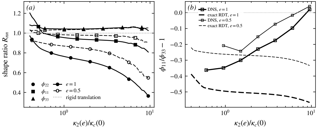
Figure 8. Exact linear theory does not translate the projected spectra rigidly. (a) Shape ratio R_{nm}(\kappa_2) of the exactly distorted, line-projected component spectra to a rigid translation under plane strain, at e = 1 (solid, filled markers) and e = 0.5 (dashed, open markers); markers distinguish the components, and the dotted line is the rigid translation R_{nm} = 1 . Closed-form Cauchy solution for an isotropic initial spectrum, integrated over the transverse wavenumber plane. (b) Transverse splitting \phi_{11}/\phi_{33} - 1 versus wavenumber in exact linear theory (dashed) and in the strained-box DNS of § 4.6 (solid, squares), at e = 1 (heavy) and e = 0.5 (light).
