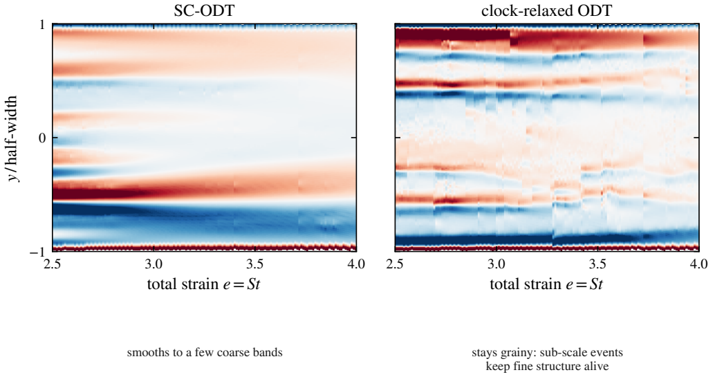
Figure S7. Small-scale (high-pass) upwash structure of a single ODT line in the high-strain window, e = 2.5\text{--}4 , in the stretched coordinate y/\text{half-width} : SC-ODT (left) against clock-relaxed ODT (right). SC-ODT smooths to a few coarse bands; the clock-relaxed line stays grainy, its sub-scale relaxation events sustaining fine-scale structure (the vertical striations are individual events). Amplitudes are normalised and the two are different realisations, so the contrast is the clock's structural signature, not a pointwise difference.
