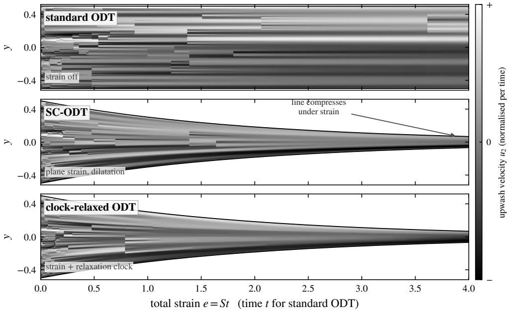
Figure S6. Space–time evolution of the ODT line, upwash velocity u_2 (normalised at each instant; blue/red or light/dark denote the sign), for standard ODT, SC-ODT and clock-relaxed ODT, advanced from matched initial fields. Time runs left to right as the total strain e = St (elapsed time for the unstrained standard-ODT case); the black envelope is the physical line half-width. Standard ODT keeps its full width; SC-ODT and clock-relaxed ODT compress under the plane strain, the clock-relaxed line retaining finer structure at high strain.
