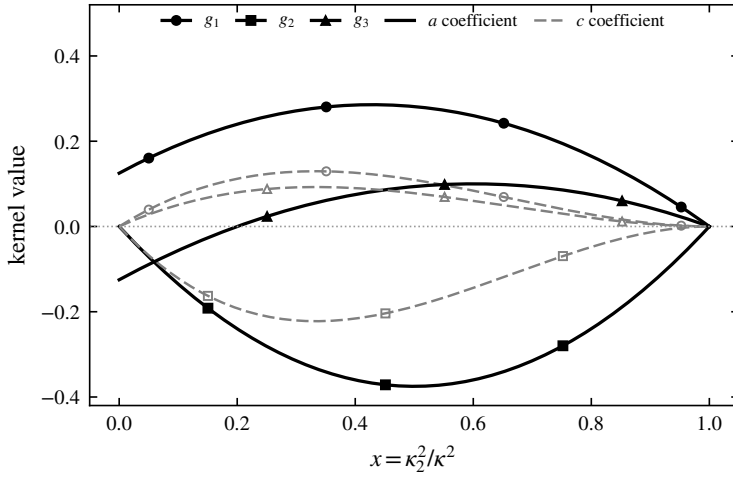
Figure 14. Rapid pressure–strain closure kernels g_1 (circles), g_2 (squares), g_3 (triangles) (eqs. (5.7)–(5.9)) against the angular variable x = \kappa_2^2/\kappa^2 . Solid curves: coefficient of the isotropic-like spectral scalar a ; faint grey dashed curves: coefficient of the anisotropy scalar c . The kernels sum to zero at every x (energy conservation, eq. (5.10)) and vanish at x = 1 . Averaged over an isotropic spectrum they give the ratio +\frac{1}{5} : -\frac{1}{5} : 0 (eq. (5.11)), recovering the isotropisation-of-production form \Pi_{ij}^{(r)} = \frac{4}{5}k_t S_{ij} (Crow 1968) that underlies the moment closure used in § 4.
