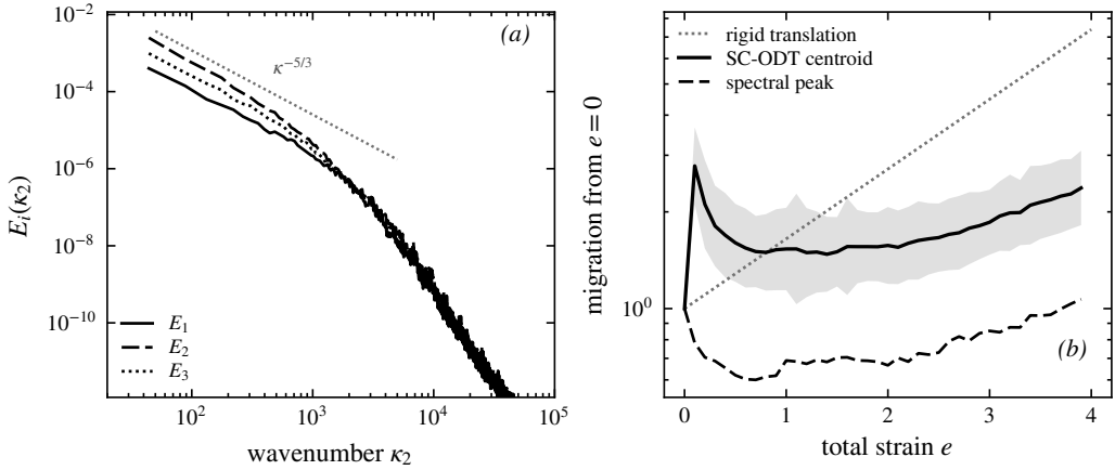
Figure 10. The physical operating point ( \nu \approx 3 \times 10^{-6} , Re_{\mathcal{L}} \approx 4.4 \times 10^3 , 16000 cells; ensemble over 200 realisations, geometric \pm\sigma ). (a) Final-strain component spectra (solid E_1 , dashed E_2 , dotted E_3 ): smooth rolloff with no grid-scale shelf; the upwash E_2 amplified above the streamwise E_1 ; grey dotted reference slope \kappa^{-5/3} . (b) Migration of the total-spectrum centroid (solid) and the spectral peak (dashed) against the rigid-translation law (grey dotted); the broadband distortion that linear theory cannot represent, at the operating point and with the noise averaged out.
