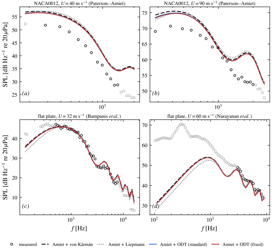
Figure 19. Absolute far-field predictions against published measurements, all four inflow spectra through the identical non-compact response (Amiet 1975; Roger & Moreau 2010): frozen von Kármán (dashed), frozen Liepmann (dotted), the computed standard-model spectrum (blue) and the computed clock-relaxed spectrum (red), each entered at the case's effective free-distortion strain. (a,b) NACA0012 of Paterson & Amiet (1976) ( c = 0.23 \text{ m} , u'_w/U \approx 4\text{--}5\% , \Lambda_f \approx 30 \text{ mm} , observer 2.25 \text{ m} overhead; Gershfeld thickness admittance applied identically to all four chains); (c) ECL flat plate of Bampanis et al. (2022) ( c = 0.10 \text{ m} , 3 \text{ mm} thick, Tu = 4.5\% , \Lambda = 9 \text{ mm} , \theta = 90^\circ , R = 1.25 \text{ m} ); (d) ISVR flat plate of Narayanan et al. (2015) ( c = 0.15 \text{ m} , Tu = 2.5\% , \Lambda = 6 \text{ mm} , R = 1.2 \text{ m} ). Black measured symbols lie in each case's stated comparison band (grey outside: background flags, facility contamination, thickness-breakdown frequency); spectra digitised from the published figures with per-figure calibration checks ( \pm 0.5 \text{ dB} ). The effective strain is a geometric estimate (potential-flow stagnation-line accumulation truncated at the eddy scale); the shaded band spans truncation at \Lambda/4\text{--}\Lambda .
