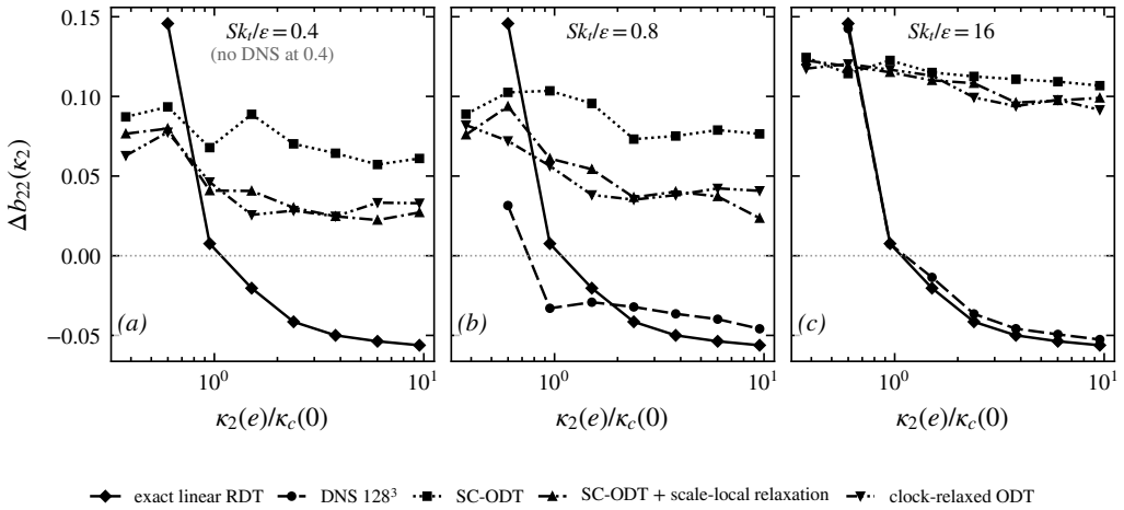
Figure 16. The five-way comparison on the benchmark observable of § 4.6.1: strain-induced upwash anisotropy per wavenumber band at e = 1 , for exact linear RDT, DNS, SC-ODT, and SC-ODT with each mechanism form—scale-local relaxation at adaptive depth, and the clock-relaxed variant (size-capped relaxation clock)—at Sk_t/\varepsilon = 0.4, 0.8 and 16 (ODT: 1024 realisations per case, same binary and precursor protocol; DNS and companions as in § 4.6; no DNS exists at 0.4 , where exact RDT is the reference—at fixed total strain it is independent of the strain rate). At rapid strain the DNS realises the exact-RDT allocation; the mechanism moves the model towards the DNS increasingly as the rapidity falls.
