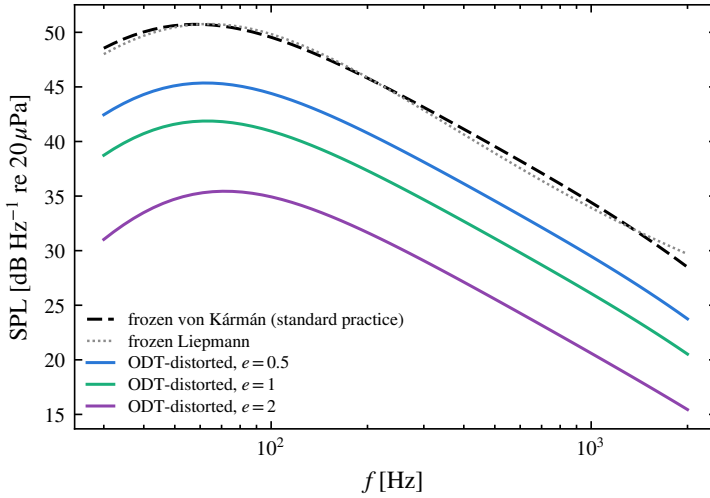
Figure 18. The assembled absolute prediction at the reference configuration of § 4.4: far-field sound pressure level from the compact lift-dipole form of Amiet (1975) with the exact Sears response, for a flat plate of chord 0.39 m ( Re_c \approx 5 \times 10^5 ) and span 0.8 m at U_\infty = 20 \text{ m s}^{-1} , u'/U_\infty = 6\% , \mathcal{L} = 55 \text{ mm} , observer 1 m overhead. Dashed: the frozen von Kármán inflow of standard practice (the e = 0 member of the fitted representation, which is exactly the isotropic von Kármán spectrum); grey dotted: the frozen Liepmann spectrum at the same (u', \mathcal{L}) , an independent analytic cross-check of the physical-unit bridge. Solid: the same chain with the computed distorted inflow at total strains e = 0.5, 1 and 2 ( Sk_t/\varepsilon \approx 0.4 ), level and shape both included.
