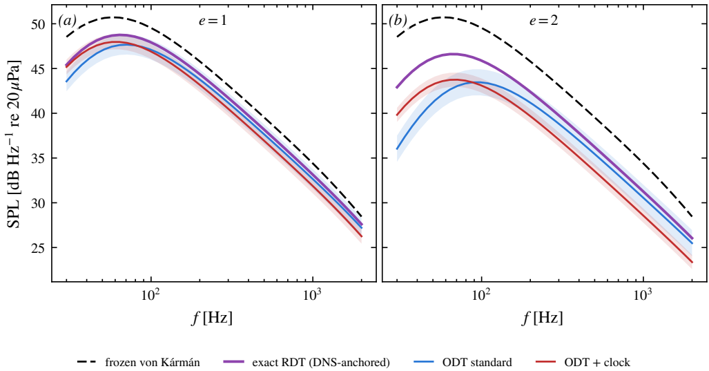
Figure 20. Computed against prescribed inflow at application strains, judged by the linear reference: absolute SPL at the reference configuration for the rapid family ( Sk_t/\varepsilon \approx 8 ) at (a) e = 1 and (b) e = 2 . Purple: exact (inviscid) RDT of the model's relaxed initial state—the reference the strained-box DNS of § 4.6 validates at rapid rates—with level set by the kernel's exact upwash amplification (reproducing the moment-level value to 0.7%). Dashed: the frozen von Kármán inflow of standard practice. Blue/red: the standard and clock-relaxed computed inflows (fitted representations, measured ensemble levels), each shaded by its measured spectral rms distance from the RDT family mapped to decibels.
