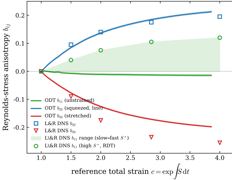
Figure 4. Reynolds-stress anisotropy under plane strain: present model (lines; ensemble mean over 1000 realisations, standard-error band) against the DNS of Lee & Reynolds (1985) (symbols, digitised from their figure 5.4). The strained components b_{22} and b_{33} are reproduced quantitatively; the unstrained b_{11} is strain-rate-dependent in the DNS (shaded band), with the model’s near-zero value at the slow-strain edge.
