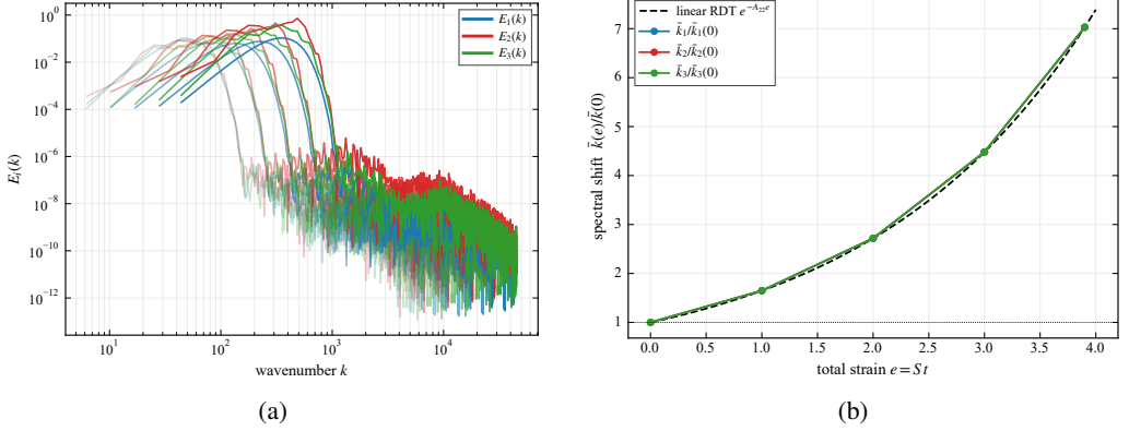
Figure 8. Compression without cascade (eddy events suppressed, inviscid). (a) Component spectra E_i(k) at increasing total strain (lighter to darker); the spectra translate to higher k without changing shape. (b) Spectral-centroid migration \bar{k}(e)/\bar{k}(0) for each component (symbols) against the kinematic prediction e^{-A_{22}e} (dashed). The centroid follows the prediction exactly and the three components coincide, confirming purely geometric compression of the line.
