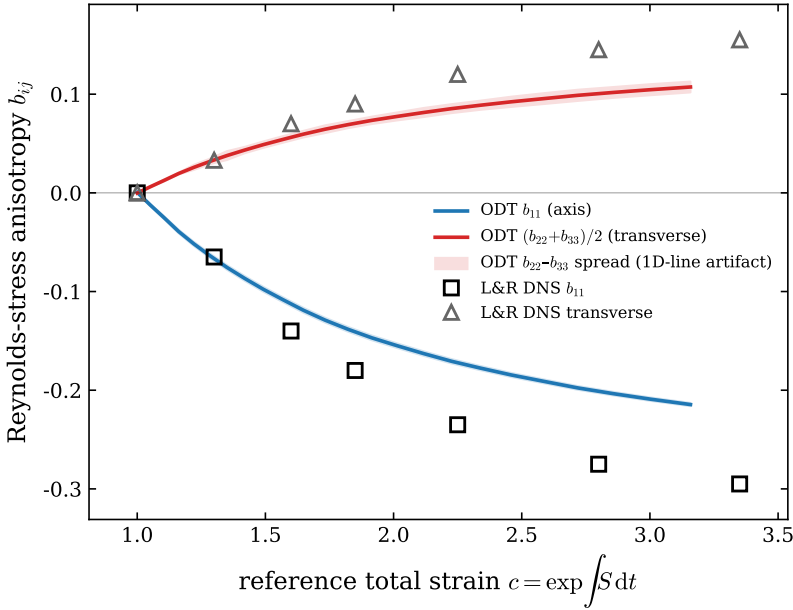
Figure 5. Anisotropy under axisymmetric contraction: present model (lines; 1000 realisations) against Lee & Reynolds (1985) (symbols, digitised from their figure 5.8). The shaded spread is the residual b_{22} \neq b_{33} split from the line’s breaking of the transverse symmetry.
