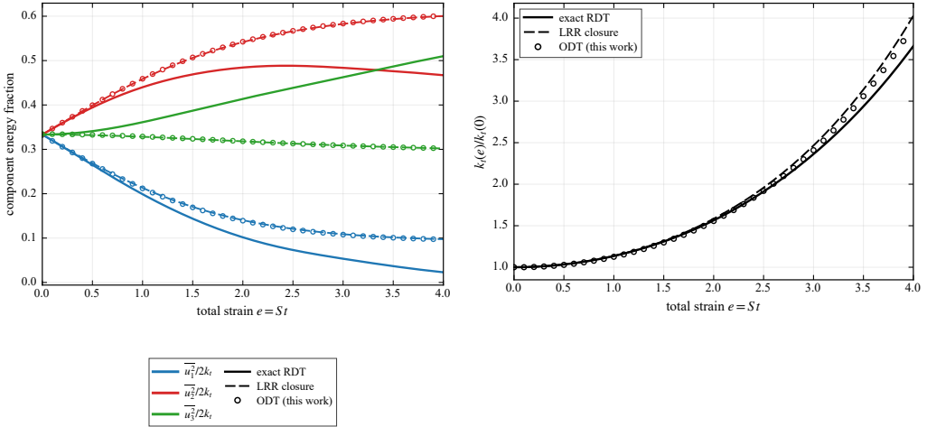
Figure 3. Verification of the strain-coupled implementation under plane strain, eddy events suppressed and zero molecular diffusion. (a) Component energy fractions; (b) kinetic-energy amplification k_t(e)/k_t(0) . Symbols: solver, length-weighted line averages. Dashed: the LRR closure integrated as a moment equation. Solid: exact rapid-distortion theory. The solver reproduces the closure to 5 \times 10^{-4} in the fractions and 0.3% in the energy; the offset from the exact solution is the closure error of § 3.2, as it must be.
