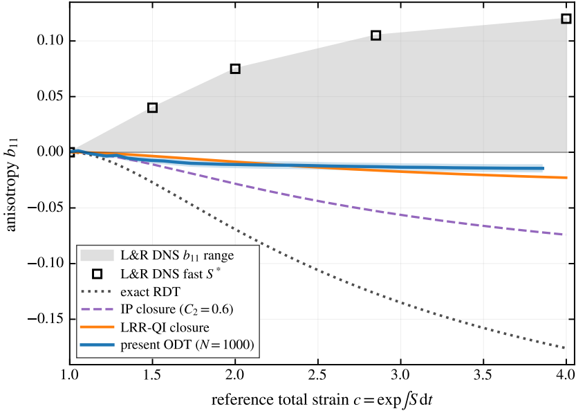
Figure 6. The unstrained-direction anisotropy b_{11} under plane strain: present model (solid, 1000 realisations, standard-error band) against exact linear rapid distortion (dotted), the IP and LRR-QI closures, and the DNS of Lee & Reynolds (1985) (symbols and shaded S^* range). The model coincides with the closure it is built on; the DNS rise to b_{11} > 0 lies above the entire closure family and reflects finite-Reynolds-number vorticity structure outside the moment-closure framework.
