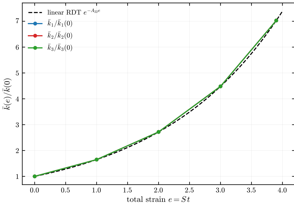
Spectral-centroid migration vs linear RDT
