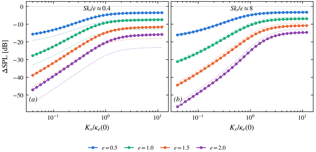
Figure 16. Change of the Amiet leading-edge-noise kernel when the frozen inflow spectrum is replaced by the computed distorted one, against reduced streamwise wavenumber, at total strains e = 0.5 – 2 : (a) Sk_t/\varepsilon \approx 0.4 , (b) \approx 8 . Solid: spectral reallocation at matched upwash variance (shape only); dotted: total, including the measured variance change ( -3.5 to -7.3 dB at the slow rate, where decay dominates the transit; +0.5 to +1.9 dB at the rapid rate, where the upwash amplification survives). Geometry, aerofoil response and observer position cancel identically in this ratio.
