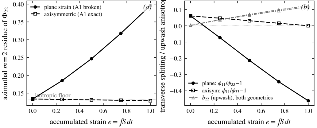
Figure 12. The A1 control experiment at Sk_t/\varepsilon = 16 ( 128^3 , four realisations): plane strain (A1 broken; solid, filled circles) against axisymmetric contraction at matched A_{22} (A1 exact by symmetry; dashed, open squares). (a) Azimuthal m = 2 residue of \Phi_{22} : it grows under plane strain but stays at the isotropic floor (grey dotted) under axisymmetric strain. (b) Transverse splitting \phi_{11}/\phi_{33} - 1 per geometry, and the upwash anisotropy b_{22} (grey dash-dot, indistinguishable between geometries)—the azimuthal structure A1 assumes away is what differs, while the acoustically relevant upwash amplification is robust.
