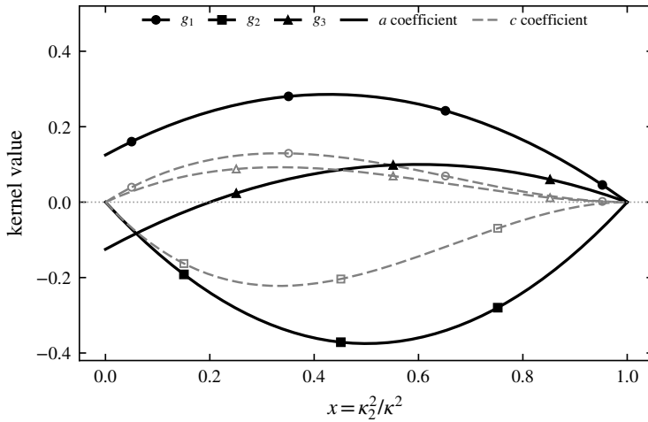
Figure 13. Rapid pressure–strain closure kernels g_1 (circles), g_2 (squares), g_3 (triangles) (eqs. (5.7)–(5.9)) against the angular variable x = \kappa_2^2 / \kappa^2 . Solid curves: coefficient of the isotropic-like spectral scalar a ; faint grey dashed curves: coefficient of the anisotropy scalar c . The kernels sum to zero at every x (energy conservation, eq. (5.10)) and vanish at x = 1 . Averaged over an isotropic spectrum they give the ratio +\frac{1}{5} : -\frac{1}{5} : 0 (eq. (5.11)), recovering the isotropisation-of-production form \Pi_{ij}^{(r)} = \frac{4}{3} k_t S_{ij} (Crow 1968) that underlies the moment closure used in § 4.
