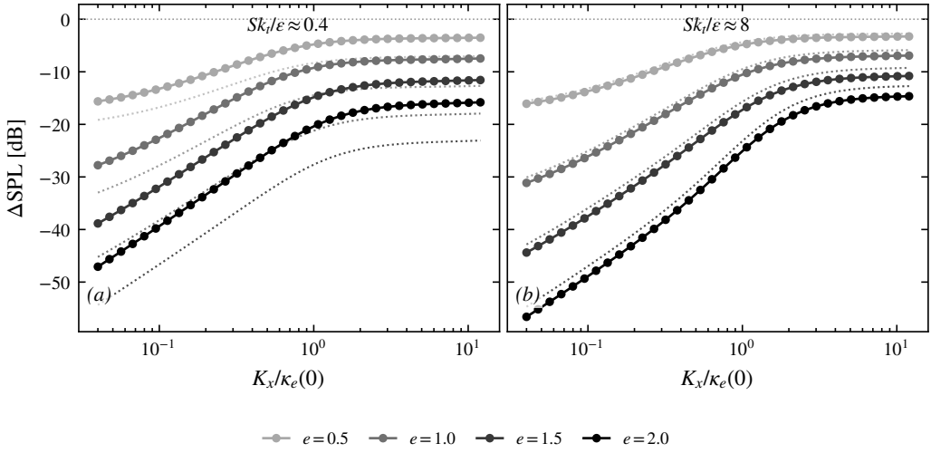
Figure 17. Change of the Amiet leading-edge-noise kernel when the frozen inflow spectrum is replaced by the computed distorted one, against reduced streamwise wavenumber, at total strains e = 0.5 – 2 (shade light to dark with increasing strain): (a) Sk_t/\varepsilon \approx 0.4 , (b) \approx 8 . Solid: spectral reallocation at matched upwash variance (shape only); dotted: total, including the measured variance change ( -3.5 to -7.3 dB at the slow rate, where decay dominates the transit time; +0.5 to +1.9 dB at the rapid rate, where the upwash amplification survives). Geometry, aerofoil response and observer position cancel identically in this ratio.
