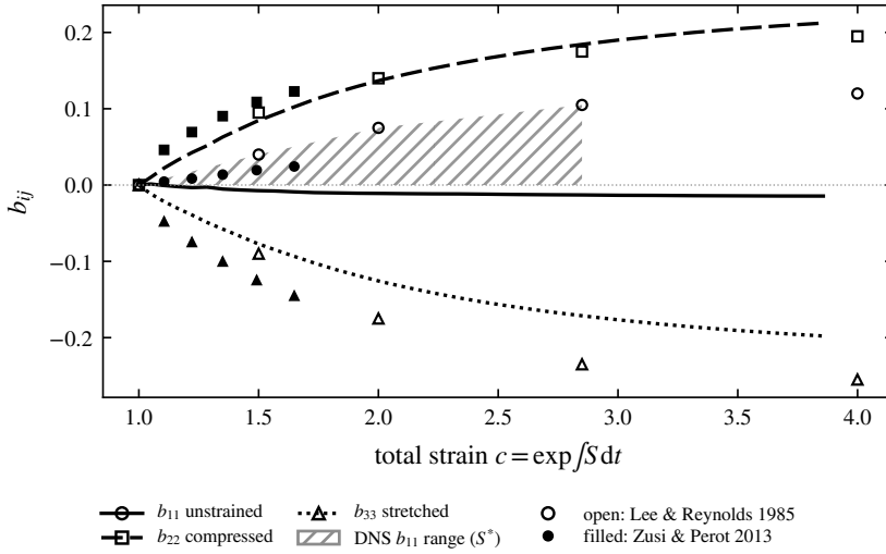
Figure 4. Reynolds-stress anisotropy under plane strain: SC-ODT (lines; ensemble mean over 1000 realisations, standard error within the line width) against the DNS of Lee & Reynolds (1985) (open symbols, digitised from their figure 5.4). As noted in § 3.3, here and henceforth all strained computations use the LRR closure. Line style and marker denote the component ( b_{11} solid/ \circ , b_{22} dashed/ \square , b_{33} dotted/ \triangle ); open markers are Lee & Reynolds (1985) , filled markers the independent DNS of Zusi & Perot (2013) (their highest rate, over the strained range c \leq 1.65 ); the hatched band is the DNS b_{11} range over slow-to-fast S^* . The strained components b_{22} and b_{33} are reproduced quantitatively, and the two DNS agree where they overlap; the unstrained b_{11} is strain-rate-dependent in the DNS, with SC-ODT at its slow-strain edge.
