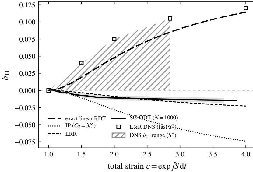
Figure 6. The unstrained-direction anisotropy b_{11} under plane strain: SC-ODT (solid, 1000 realisations, grey standard-error band) against exact linear rapid distortion (long-dashed, wavevector-ensemble integration), the IP (dotted) and LRR (short-dashed) closures, and the DNS of Lee & Reynolds (1985) (open squares; hatched band = DNS range over slow-to-fast S^* ). The fast-strain DNS tracks exact RDT, whose rapid pressure-strain feeds the neutral direction; the single-point closures—and SC-ODT, built on them—miss this orientation-carried redistribution, the deficiency measured and localised in § 5.6.
