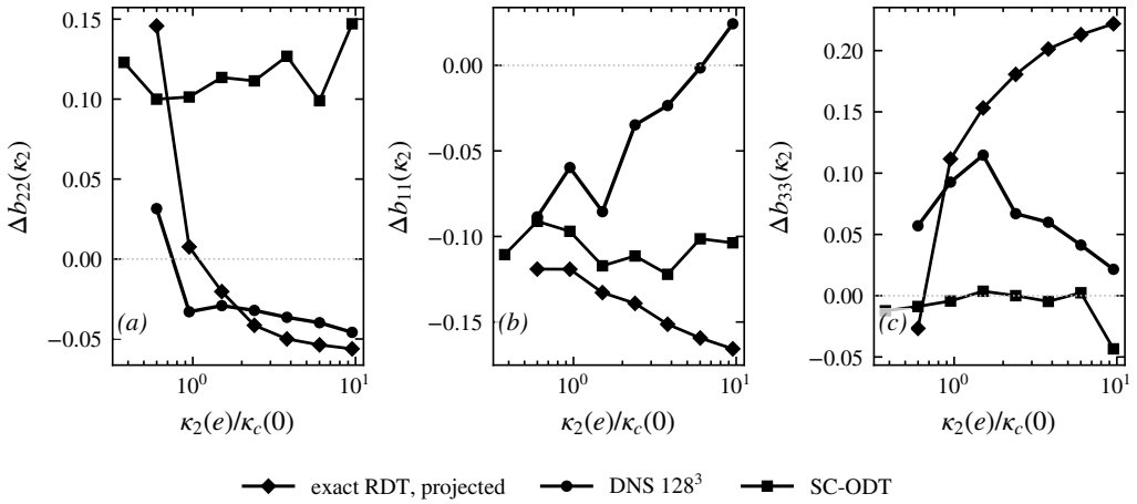
Figure 11. Three-way comparison at e = 1 , Sk_t/\varepsilon = 0.8 : strain-induced anisotropy of the line spectra relative to each system's own unstrained state, resolved by component—(a) \Delta b_{22} , (b) \Delta b_{11} , (c) \Delta b_{33} . SC-ODT (■, 1024 realisations) against exact projected RDT (♦) and DNS ( 128^3 , ●, four realisations). The SC-ODT curves are relatively flat in every panel—the wavenumber-uniform signature—whereas exact RDT and the DNS vary with wavenumber.
