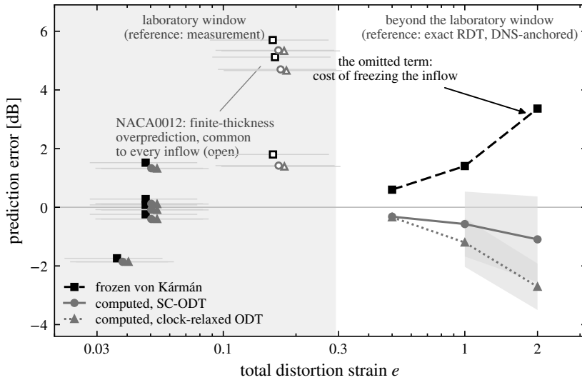
Figure 21. The cost of the frozen-inflow assumption against accumulated distortion: signed far-field prediction error, judged by the best available reference at each strain. Laboratory window (shaded): the eight measured cases of figure 19, bias over each case’s comparison band—flat plates filled, NACA0012 open (its common overprediction is the finite-thickness effect); horizontal bars span the effective-strain truncation range, and the three inflow chains are offset slightly in e for legibility. Beyond the window: band-mean error over 100–1000 Hz against the exact-RDT reference of figure 20 at e = 0.5, 1 and 2 ; shaded bands give the \pm 10 \log_{10}(1 + \text{rms}) spectral-distance uncertainty where measured ( e = 1, 2 ).
