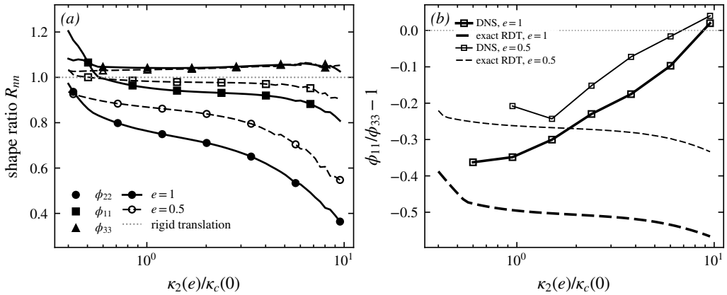
Figure 8. Exact linear theory does not translate the projected spectra rigidly. (a) Shape ratio R_{nn}(\kappa_2) of the exactly distorted, line-projected component spectra to a rigid translation under plane strain, at e = 1 (solid, filled markers) and e = 0.5 (dashed, open markers); markers distinguish the components, and the dotted line is the rigid translation R_{nn} = 1 . Closed-form Cauchy solution for an isotropic initial spectrum, integrated over the transverse wavenumber plane. (b) Transverse splitting \phi_{11}/\phi_{33} - 1 versus wavenumber in exact linear theory (dashed) and in the strained-box DNS of § 4.6 (solid, squares), at e = 1 (heavy) and e = 0.5 (light).
