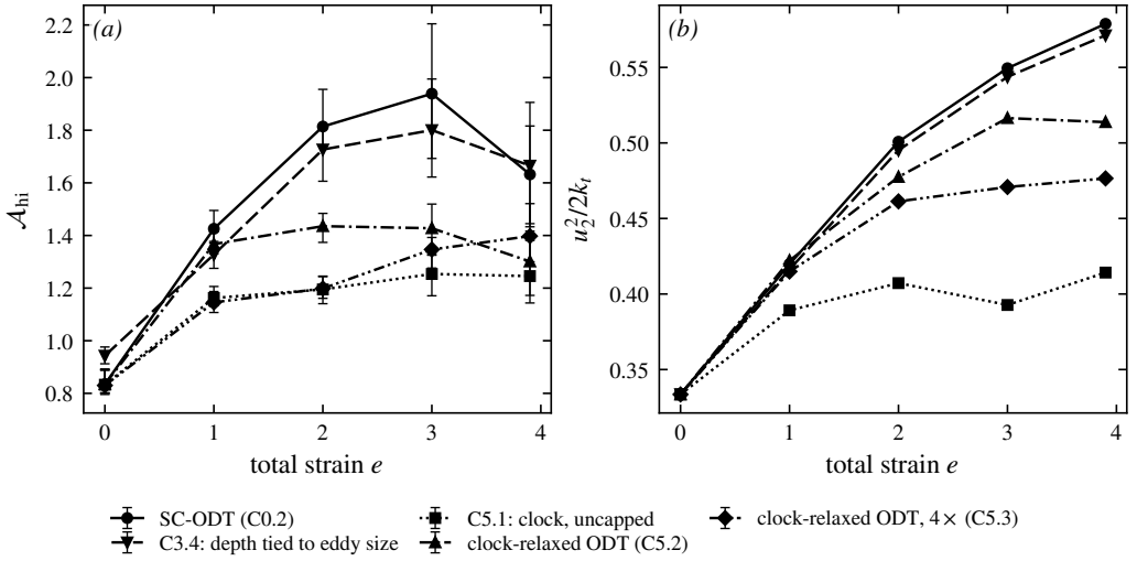
Figure 15. The independent relaxation clock (C5) against the eddy-locked categories. (a) Fine-scale-band imbalance \mathcal{A}_{hi} against total strain: the eddy-locked variants fade beyond e \approx 3 ; the clock holds at every strain. (b) The price: upwash energy fraction. The comparison is the SC-ODT (C0.2) trajectory—the moment-level behaviour validated in § 3.4—which the uncapped clock suppresses; the size cap at matched rate preserves it, and the 4 \times rate (C5.3) reduces it in proportion. Medians over 1024 paired-seed realisations; the clock rate is matched to the SC-ODT eddy rate.
