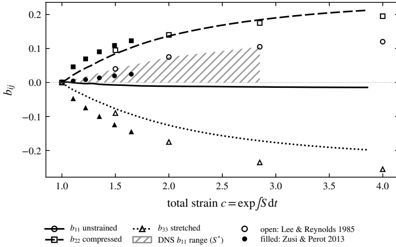
Figure 4. Reynolds-stress anisotropy under plane strain: SC-ODT (lines; ensemble mean over 1000 realisations, standard-error-band standard error within the line width ) against the DNS of Lee & Reynolds (1985) (open symbols, digitised from their figure 5.4). As noted in § 3.3, here and henceforth all strained computations use the LRR closure. Line style and marker denote the component ( b_{11} solid/ \circ , b_{22} dashed/ \square , b_{33} dotted/ \triangle ); open markers are Lee & Reynolds (1985), filled markers the independent DNS of Zusi & Perot (2013) (their highest rate, over the strained range c \leq 1.65 ); the hatched band is the DNS b_{11} range over slow-to-fast S^* . The strained components b_{22} and b_{33} are reproduced quantitatively, and the two DNS agree where they overlap; the unstrained b_{11} is strain-rate-dependent in the DNS, with SC-ODT at its slow-strain edge.
