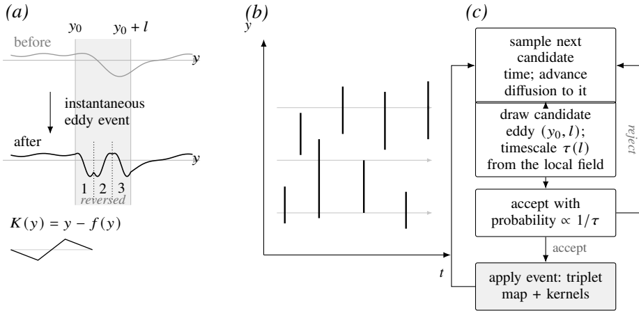
Figure 1. The model at a glance. (a) Eddy event on [y_0, y_0 + l] : triplet map + kernel K(y) redistribute energy among components while conserving momentum and total energy. (b) Instantaneous eddy events (Poisson) interleaved with diffusion and continuous mean-strain forcing. (c) Advancement cycle; the k^{-5/3} cascade emerges from repeated sampling.
