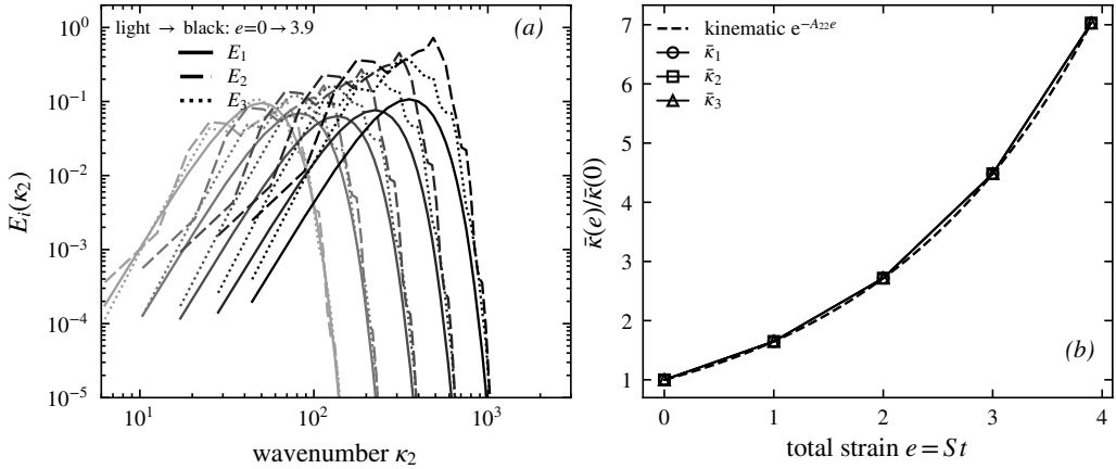
Figure 8. Compression without cascade (eddy events suppressed, inviscid). (a) Component line spectra E_i(k_2) at total strains e = 0, 1, 2, 3, 3.9 (lighter to darker); the spectra translate to higher wavenumber without changing shape. (b) Spectral-centroid migration \bar{\kappa}(e)/\bar{\kappa}(0) for each component (symbols) against the kinematic prediction e^{-A_{22}e} (dashed). The centroid follows the prediction and the three components coincide, confirming purely geometric compression of the line.
