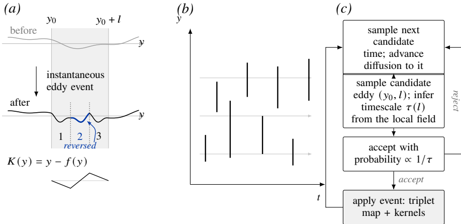
Figure 1. The model at a glance. (a) Eddy event on [y_0, y_0 + l] : the triplet map + compresses and triplicates the local field; the additive kernel K(y) redistribute- redistributes energy among components while, both conserving momentum and total energy. (b) Instantaneous eddy Eddy events (Poisson) interleaved with, the vertical bars marking the spatial range of each event, punctuating the continuous diffusion and continuous-mean-strain forcing (grey arrows). (c) Advancement cycle at a state-dependent rate; the k^{-5/3} cascade emerges from-as an outcome of repeated sampling, consistent with inertial-range phenomenology.
