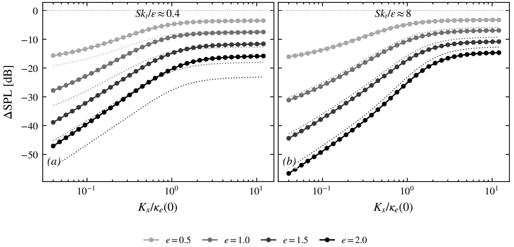
Figure 18. Change of the Amiet leading-edge-noise kernel when the frozen inflow spectrum is replaced by the computed distorted one, against reduced streamwise wavenumber, at total strains e = 0.5 – 2 (shade light to dark with increasing strain): (a) Sk_t/\varepsilon \approx 0.4 , (b) \approx 8 . Solid: spectral reallocation at matched upwash variance (shape only); dotted: total, including the measured variance change ( -3.5 to -7.3 dB at the slow rate, where decay dominates the transit; +0.5 to +1.9 dB at the rapid rate, where the upwash amplification survives). Geometry, aerofoil response and observer position cancel identically in this ratio.
