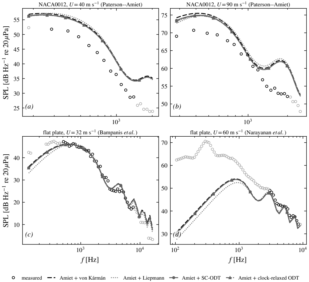
Figure 20. Absolute far-field predictions against published measurements, all four inflow spectra through the identical non-compact response (Amiet 1975; Roger & Moreau 2010): frozen von Kármán (black dashed), frozen Liepmann (grey dotted), the computed SC-ODT spectrum (grey, circles) and the computed clock-relaxed ODT spectrum (grey, triangles), each entered at the case’s effective free-distortion strain. (a,b) NACA0012 of Paterson & Amiet (1976) ( c = 0.23 m, u'_w/U \approx 4\text{--}5\% , \Lambda_f \approx 30 mm, observer 2.25 m overhead; Gershfeld thickness admittance applied identically to all four chains); (c) ECL flat plate of Bampanis et al. (2022) ( c = 0.10 m, 3 mm thick, Tu = 4.5\% , \Lambda = 9 mm, \Theta = 90^\circ , R = 1.25 m); (d) ISVR flat plate of Narayanan et al. (2015) ( c = 0.15 m, Tu = 2.5\% , \Lambda = 6 mm, R = 1.2 m). Black measured symbols lie in each case’s stated comparison band (grey outside: background flags, facility contamination, thickness-breakdown frequency); spectra digitised from the published figures with per-figure calibration checks ( \pm 0.5 dB). The effective strain is a geometric estimate (potential-flow stagnation-line accumulation truncated at the eddy scale); the shaded band spans truncation at \Lambda/4\text{--}\Lambda .
