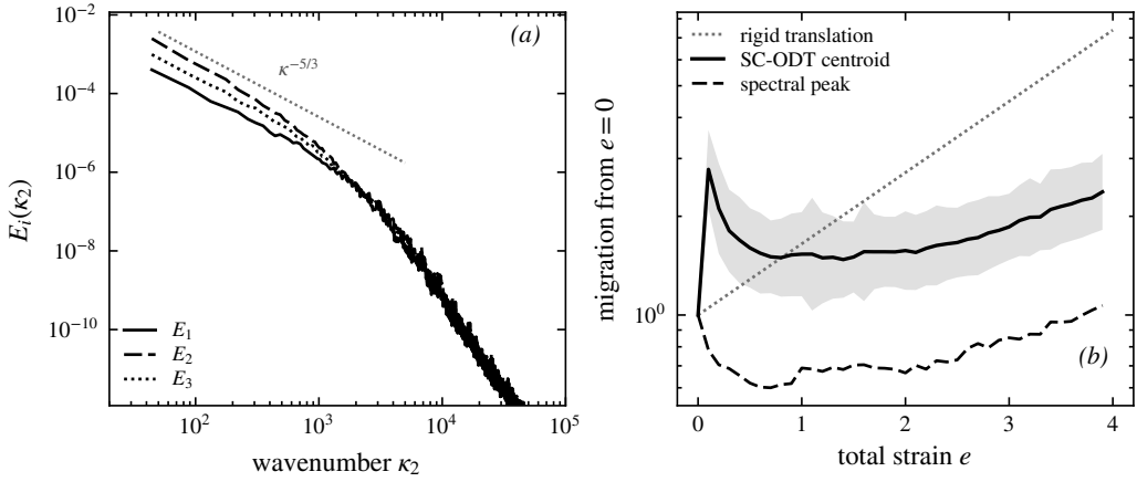
Figure 11. The physical operating point ( \nu \approx 3 \times 10^{-6} , Re_{\mathcal{L}} \approx 4.4 \times 10^3 , 16000 cells; ensemble over 200 realisations, geometric \pm\sigma ). (a) Final-strain component spectra (solid E_1 , dashed E_2 , dotted E_3 ): smooth rolloff with no grid-scale shelf; the upwash E_2 amplified above the streamwise E_1 ; grey dotted reference slope \kappa^{-5/3} . (b) Migration of the total-spectrum centroid (solid) and the spectral peak (dashed) against the rigid-translation law (grey dotted), with the geometric \pm\sigma ensemble spread shaded: the broadband distortion that linear theory cannot represent, at the operating point and with the noise averaged out.
