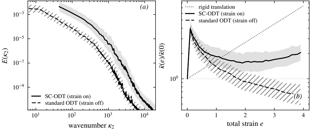
Figure 10. SC-ODT (strain on) against the matched strain-off baseline, standard ODT, at \nu = 10^{-5} (ensemble means over 128 realisations, geometric \pm\sigma bands). (a) Final-strain total spectrum E(\kappa_2) : SC-ODT (strain on, solid) extends to higher wavenumber than the baseline (strain off, dashed) but remains broadband, not a rigid translation. (b) Centroid migration: the baseline relaxes below unity, SC-ODT is lifted above it by the compression, yet stays far below the rigid-translation line (grey dotted). The gap between the strain-on and strain-off curves is the distortion attributable to the mean strain at this Reynolds number.
