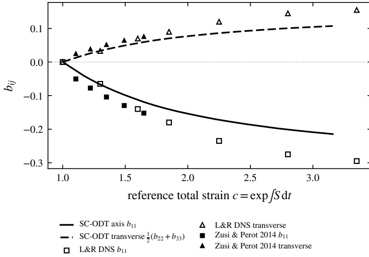
Figure 6. Reynolds-stress anisotropy under axisymmetric contraction: SC-ODT (lines; ensemble mean over 1000 realisations, standard-error band) against the DNS of Lee & Reynolds (1985) (open markers) and the independent DNS of Zusi & Perot (2014) (filled markers, their highest rate, over c \leq 1.65 ). Solid/ \square : the compressed axial component b_{11} ; dashed/ \triangle : the transverse component \frac{1}{2}(b_{22} + b_{33}) . The model tracks the sign and monotonic growth of both, and the two DNS agree where they overlap.
