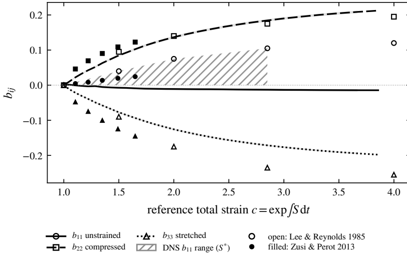
Figure 5. Reynolds-stress anisotropy under plane strain: SC-ODT (lines; ensemble mean over 1000 realisations, standard-error band) against the DNS of Lee & Reynolds (1985) (open symbols, digitised from their figure 5.4). Line style and marker denote the component ( b_{11} solid/o, b_{22} dashed/□, b_{33} dotted/△); open markers are Lee & Reynolds (1985) , filled markers the independent DNS of Zusi & Perot (2013) (their highest rate, over the strained range c \leq 1.65 ); the hatched band is the DNS b_{11} range over slow-to-fast S^* . The strained components b_{22} and b_{33} are reproduced quantitatively, and the two DNS agree where they overlap; the unstrained b_{11} is strain-rate-dependent in the DNS, with SC-ODT at its slow-strain edge.
