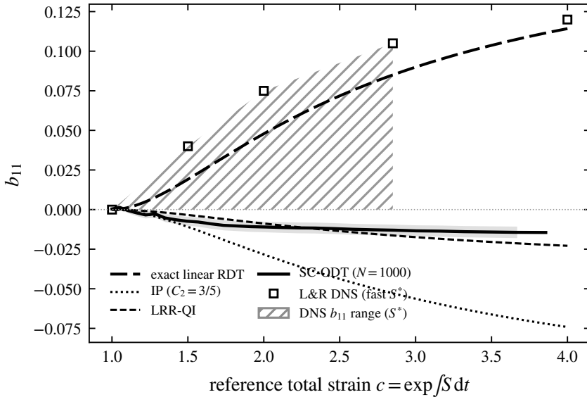
Figure 7. The unstrained-direction anisotropy b_{11} under plane strain: SC-ODT (solid, 1000 realisations, standard-error band) against exact linear rapid distortion (long-dashed, wavevector-ensemble integration), the IP (dotted) and LRR-QI (short-dashed) closures, and the DNS of Lee & Reynolds (1985) (open squares; hatched band = DNS range over slow-to-fast S^* ). The fast-strain DNS tracks exact RDT, whose rapid pressure-strain feeds the neutral direction; the single-point closures—and SC-ODT, built on them—miss this orientation-carried redistribution, the deficiency measured and localised in § 5.6.
