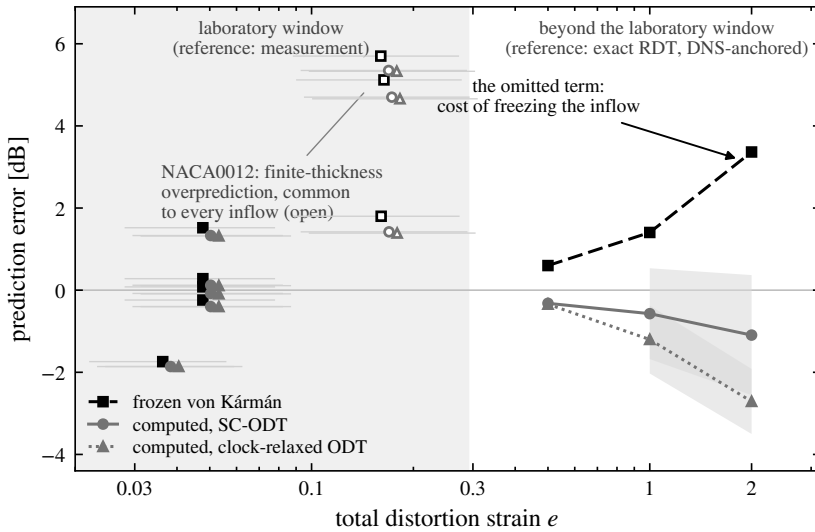
Figure 22. The cost of the frozen-inflow assumption against accumulated distortion: signed far-field prediction error, judged by the best available reference at each strain. Laboratory window (shaded): the eight measured cases of figure 20, bias over each case’s comparison band—flat plates filled, NACA0012 open (its common overprediction is the finite-thickness effect); horizontal bars span the effective-strain truncation range, and the three inflow chains are offset slightly in e for legibility. Beyond the window: band-mean error over 100–1000 Hz against the exact-RDT reference of figure 21 at e = 0.5, 1 and 2 ; shaded bands give the \pm 10 \log_{10}(1 + \text{rms}) spectral-distance uncertainty where measured ( e = 1, 2 ).
