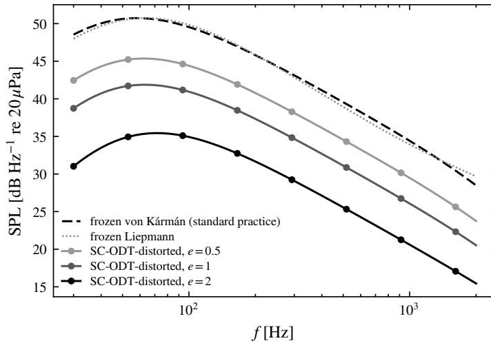
Figure 19. The assembled absolute prediction at the reference configuration of § 4.4: far-field sound pressure level from the compact lift-dipole form of Amiet (1975) with the exact Sears response (Sears 1941), for a flat plate of chord 0.39 m ( Re_c \approx 5 \times 10^5 ) and span 0.8 m at U_\infty = 20 \text{ m s}^{-1} , u'/U_\infty = 6\% , \mathcal{L} = 55 \text{ mm} , observer 1 m overhead. Dashed: the frozen von Kármán inflow of standard practice (the e = 0 member of the fitted representation, which is exactly the isotropic von Kármán spectrum); grey dotted: the frozen Liepmann spectrum at the same ( u' , \mathcal{L} ), an independent analytic cross-check of the physical-unit bridge. Solid (grey light to black with increasing strain, circles): the same chain with the SC-ODT-distorted inflow at total strains e = 0.5, 1 and 2 ( Sk_t/\varepsilon \approx 0.4 ), level and shape both included.
