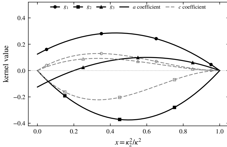
Figure 15. Rapid pressure–strain closure kernels g_1 (circles), g_2 (squares), g_3 (triangles) (eqs. (5.7)–(5.9)) against the angular variable x = \kappa_2^2 / \kappa^2 . Solid curves: coefficient of the isotropic-like spectral scalar a ; faint grey dashed curves: coefficient of the anisotropy scalar c . The kernels sum to zero at every x (energy conservation, eq. (5.10)) and vanish at x = 1 . Averaged over an isotropic spectrum they give the ratio +\frac{1}{5} : -\frac{1}{5} : 0 (eq. (5.11)), recovering the isotropisation-of-production form \Pi_{ij}^{(r)} = \frac{4}{5} k_t S_{ij} (Crow 1968) that underlies the moment closure used in § 4.
