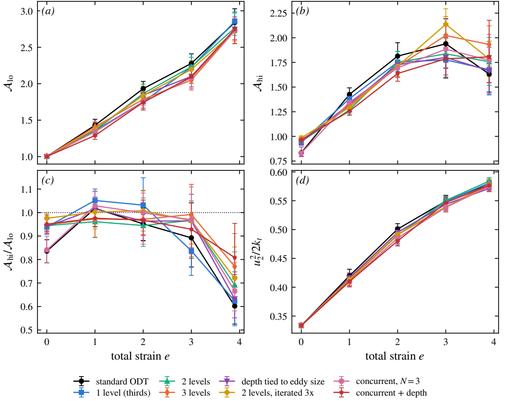
Figure 17. Scale-local relaxation on the transmission diagnostic: (a) energy-containing-band imbalance \mathcal{A}_{lo} , (b) fine-scale-band imbalance \mathcal{A}_{hi} , (c) transmission \mathcal{A}_{hi}/\mathcal{A}_{lo} , (d) upwash energy fraction, against total strain: standard ODT, hierarchical sub-scale kernels at fixed depth (1–3 levels), depth tied to eddy size, the per-event iterated variant, concurrent relaxation ( N = 3 randomly placed same-size intervals per event), and the stacked variant (concurrent intervals each running the adaptive hierarchy). Medians over 1024 paired-seed realisations, 95% bootstrap intervals.
