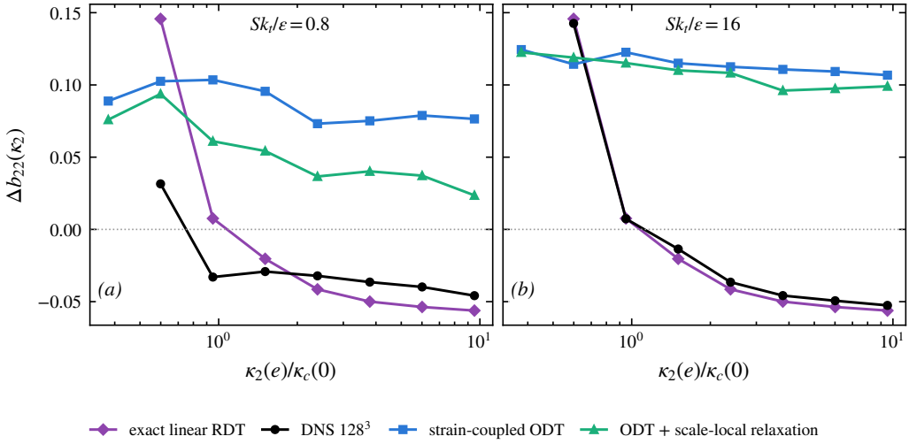
Figure 18. The four-way comparison on the benchmark observable of § 4.2.1: strain-induced upwash anisotropy per wavenumber band at e = 1 , for exact linear RDT, DNS, the strain-coupled model, and the model with adaptive-depth scale-local relaxation, at (a) Sk_t/\varepsilon = 0.8 and (b) 16 (ODT: 1024 realisations per case, same binary and precursor protocol; DNS and companions as in § 4.2). At rapid strain the DNS realises the exact-RDT allocation; scale-local relaxation moves the model towards the DNS at moderate rapidity and only marginally at rapid strain.
