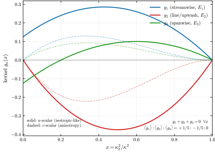
Figure 6. Rapid pressure–strain closure kernels g_1, g_2, g_3 (eqs. (5.8)–(5.10)) against the angular variable x = \kappa_2^2/\kappa^2 . Solid curves: coefficient of the isotropic-like spectral scalar a ; faint dashed curves: coefficient of the anisotropy scalar c . The kernels sum to zero at every x (energy conservation, eq. (5.11)) and vanish at x = 1 . Averaged over an isotropic spectrum they give the ratio +\frac{1}{5} : -\frac{1}{5} : 0 (eq. (5.12)), recovering the isotropisation-of-production form \Pi_{ij}^{(r)} = \frac{4}{3}k_t S_{ij} (Crow 1968) that underlies the moment closure used in § 4.
