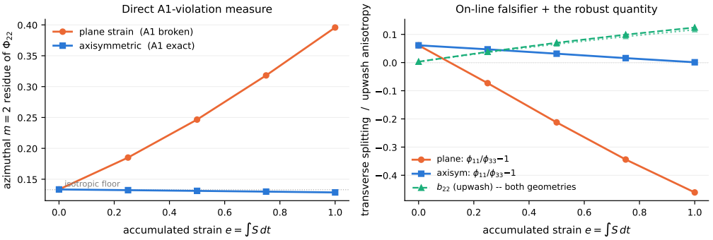
Figure 5. The A1 control experiment at Sk_t/\varepsilon = 16 (128 3 , four realisations): axisymmetric contraction (A1 exact by symmetry) against plane strain at matched A_{22} . Left: azimuthal m = 2 residue of \Phi_{22} . Right: transverse splitting and b_{22} .
