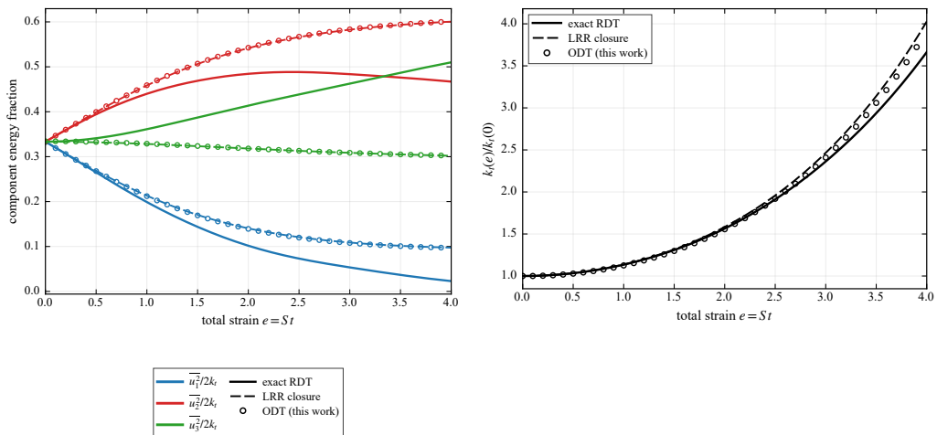
Figure 3. Verification of the strain-coupled ODT implementation under plane strain, with eddy events suppressed and zero molecular diffusion. (a) Component energy fractions \overline{u_i^2}/2k_t (colour denotes the component); (b) turbulent kinetic energy amplification k_t(e)/k_t(0) . Symbols: ODT solver, length-weighted line averages at the output times. Dashed: the LRR closure (4.5) integrated as a moment equation. Solid: exact rapid-distortion theory. The solver reproduces the LRR closure in the fractions (to 5 \times 10^{-4} ) and in the energy amplification (to within 3%); the residual energy deficit at large strain is interpolation loss from the adaptive mesh under-resolving the strained fine scales, and is addressed in § 4.2.
