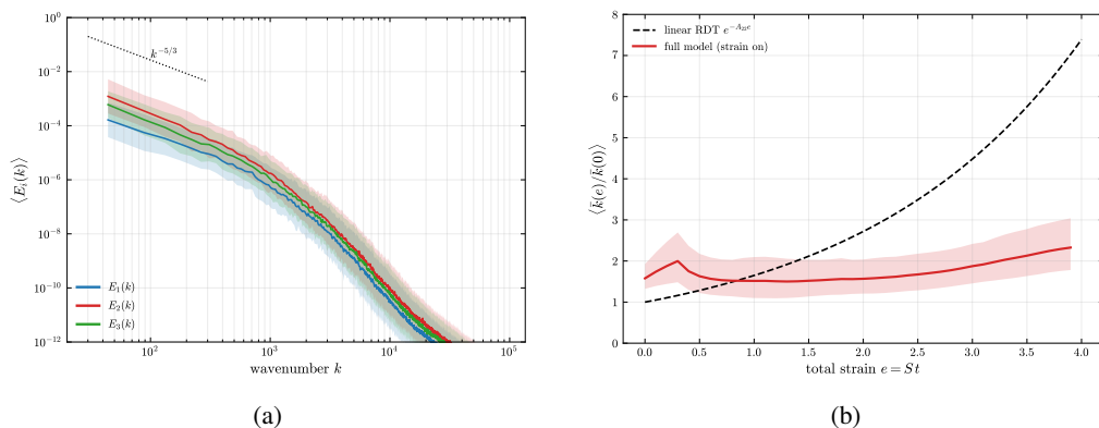
Figure 9. Physical operating point \nu \approx 3 \times 10^{-6} ( Re_{\mathcal{L}} \approx 4.4 \times 10^3 ), resolved on a 16000-cell grid; ensemble means over N = 200 realisations with geometric \pm\sigma bands. (a) Final-strain component spectra \langle E_i(k) \rangle : the resolved spectrum falls smoothly across four decades with no grid-scale shelf; the upwash component E_2 (red) is amplified above the streamwise E_1 (blue). The dotted line marks a k^{-5/3} slope. (b) Total-spectrum centroid migration \langle \bar{k}(e) \rangle / \bar{k}(0) (the centroid curve lightly smoothed) against the linear-RDT prediction e^{-A_{22}e} (dashed). After the initialisation transient near e \approx 0.3 , the centroid migrates to \approx 2.4 by e = 4 , far below the rigid-translation value of 7.4: the broadband distortion that linear theory cannot represent.
