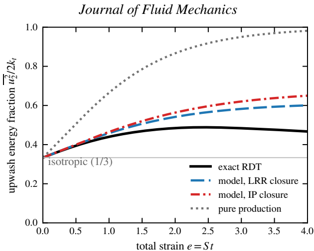
Figure 2. Upwash energy fraction \overline{u_2^2}/2k_t against total strain under plane strain, for initially isotropic turbulence. Black: exact rapid-distortion theory; blue dashed: present model with the LRR closure; red dash-dotted: present model with the IP closure; grey dotted: production alone ( B_{ij} = 0 ). Production without the rapid pressure-strain overstates the onset amplification rate by \frac{5}{2} and forces almost all the energy into the upwash component; the rapid term restores the physical, bounded amplification.
