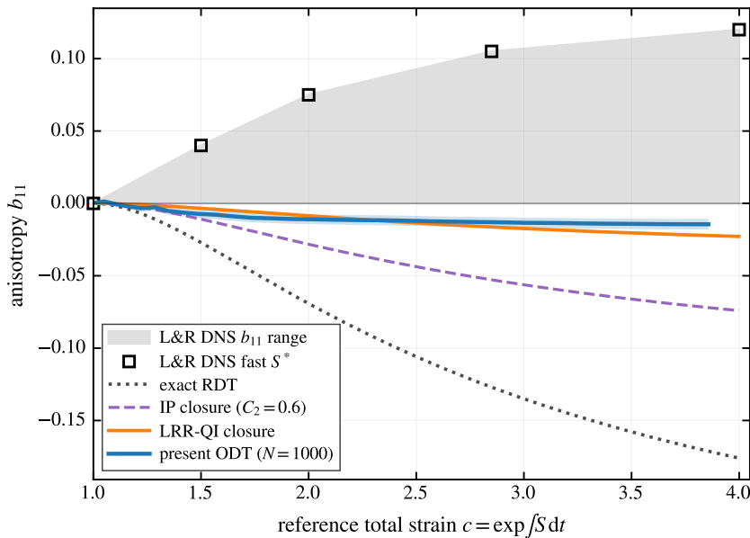
Figure 14. The unstrained-direction anisotropy b_{11} under plane strain: the present ODT (solid, N = 1000 , with standard-error band) compared with exact linear rapid-distortion theory (dotted), the isotropization-of-production closure (dashed), the quasi-isotropic Launder–Reece–Rodi closure (the form coded in the model), and the DNS of Lee & Reynolds (1985) (symbols and shaded S^* range). The present model coincides with the LRR-QI closure prediction; exact rapid distortion gives b_{11} < 0 , since the unstrained component is conserved while the energy grows. The DNS rise to b_{11} > 0 lies above the entire closure family and reflects finite-Reynolds-number vorticity structure outside the moment-closure framework.
