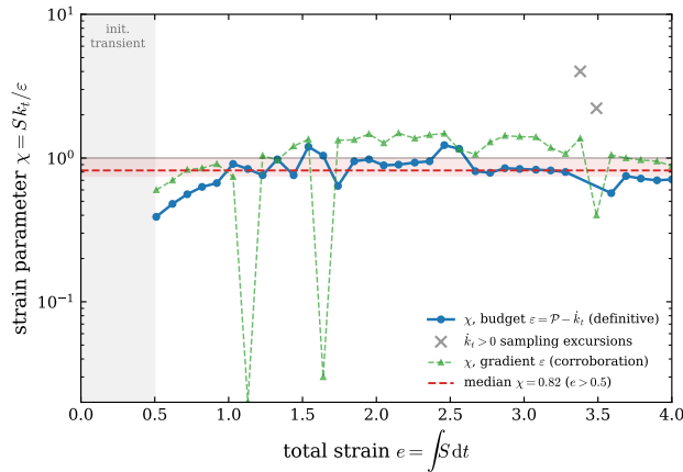
Figure 7. Strain parameter \chi = Sk_t/\varepsilon along the strained trajectory at the physical operating point ( \nu \approx 3 \times 10^{-6} , N = 200 ). The dissipation is evaluated from the resolved energy budget \varepsilon = \mathcal{P} - dk_t/dt (blue, definitive), with the gradient estimate \langle 2\nu(\partial u_i/\partial y)^2 \rangle shown for corroboration (green). After the initialisation transient (shaded, e \lesssim 0.5 ), \chi settles at \approx 0.8 (dashed line; interquartile band 0.7–0.9 shaded) and remains there to e = 4 . Crosses mark single-dump excursions in which an eddy event fires near a dump time and momentarily renders dk_t/dt positive (finite-difference sampling artefacts). The budget and gradient estimates bracket \chi = O(1) —the regime in which neither the rapid-distortion nor the near-equilibrium limit is uniformly valid, and the regime the leading-edge stagnation flow occupies.
