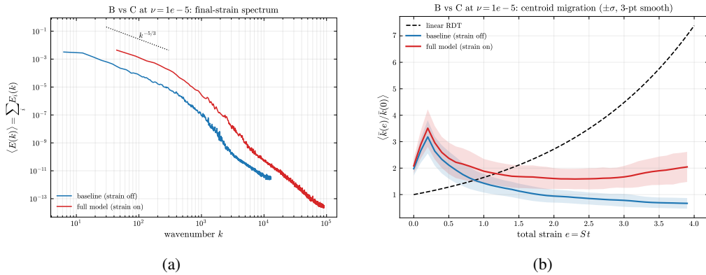
Figure 5. Full model versus matched no-strain baseline at \nu = 10^{-5} (ensemble means, N = 100 , \pm\sigma band; centroid curves lightly smoothed). (a) Final-strain spectrum E(k) = \sum_i E_i(k) : the full model (strain on) extends to higher wavenumber than the baseline (strain off) but remains broadband, not a rigid translation. (b) Centroid migration: the baseline relaxes below unity, the full model is lifted above it by the compression, yet stays far below the linear-RDT line (dashed). The gap between the two solid curves is the distortion attributable to the mean strain at this Reynolds number.
