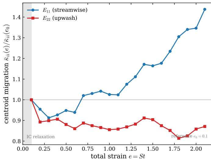
Figure 11. Full model (eddies and viscosity active; ensemble mean, N = 64 ): centroid migration of the streamwise ( E_{11} ) and upwash ( E_{22} ) component spectra, each normalised to the relaxed reference state e_0 = 0.1 . The band-limited initial field relaxes over the first strain increment (shaded); thereafter the components diverge under strain—the streamwise component migrating to higher wavenumber while the upwash component is held back—reproducing the qualitative departure-from-RDT mechanism of Chen et al. (2006) . The comparison is qualitative; see text.
