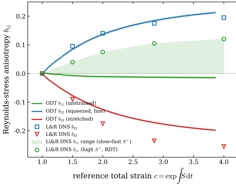
Figure 12. Reynolds-stress anisotropy under plane strain: present model (lines; ensemble mean over N = 1000 realizations, standard-error band shown) versus the DNS of Lee & Reynolds (1985) (symbols, digitised from their Figure 5.4). The compressed component b_{22} and stretched component b_{33} are reproduced quantitatively. The unstrained component b_{11} is strongly strain-rate-dependent in the DNS; its range from slow to fast strain rate is shown as the shaded band, with the model's near-zero value lying at the slow-strain edge. Reference total strain c = \exp \int S dt .
