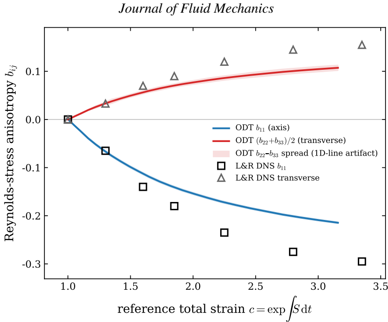
Figure 13. Reynolds-stress anisotropy under axisymmetric contraction: present model (lines; N = 1000 ) versus the DNS of Lee & Reynolds (1985) (symbols, digitised from their Figure 5.8). The axis component b_{11} and the transverse mean \frac{1}{2}(b_{22} + b_{33}) are compared; the shaded spread is the residual b_{22} \neq b_{33} split arising because the one-dimensional line breaks the transverse symmetry of the flow. The model reproduces the trend and sign structure while under-predicting the anisotropy magnitude by about 25%.
