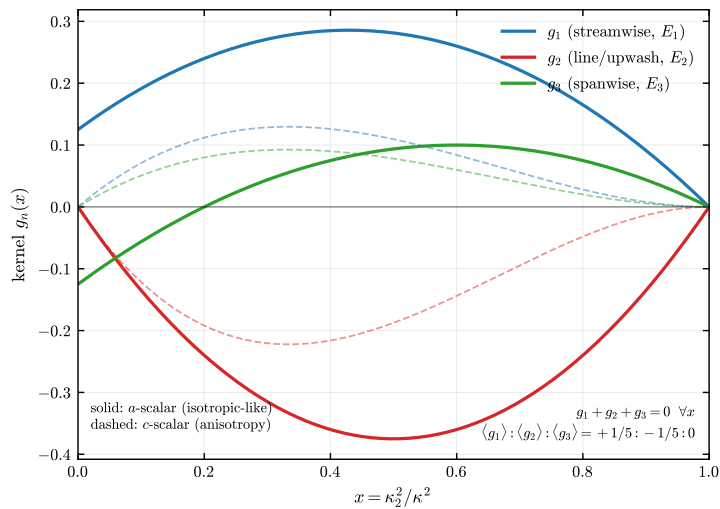
Figure 15. Rapid pressure–strain closure kernels g_1, g_2, g_3 (eqs. (5.8)–(5.10)) against the angular variable x = \kappa_2^2/\kappa^2 . Solid curves: coefficient of the isotropic-like spectral scalar a ; faint dashed curves: coefficient of the anisotropy scalar c . The kernels sum to zero at every x (energy conservation, eq. (5.11)) and vanish at x = 1 . Averaged over an isotropic spectrum they give the ratio +1/5 : -1/5 : 0 (eq. (5.12)), recovering the isotropisation-of-production form \Pi_{ij}^{(r)} = \frac{4}{3}k_t S_{ij} (Crow 1968) that underlies the moment closure used in § 4.2.
