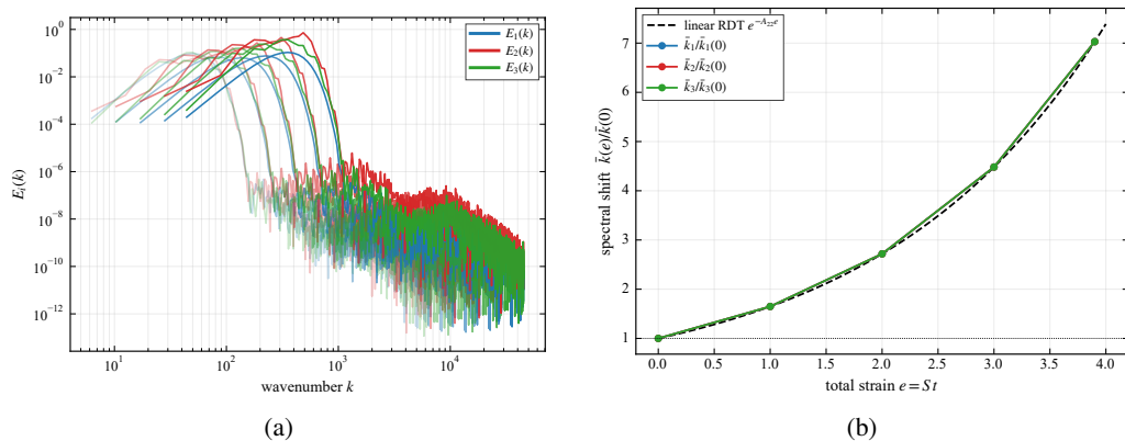
Figure 4. Compression without cascade (eddy events suppressed, inviscid). (a) Component spectra E_i(k) at increasing total strain (lighter to darker); the spectra translate to higher k without changing shape. (b) Spectral-centroid migration \bar{k}(e)/\bar{k}(0) for each component (symbols) against the linear-RDT prediction e^{-A_{22}e} (dashed). The centroid follows the prediction exactly and the three components coincide, confirming purely geometric compression.
