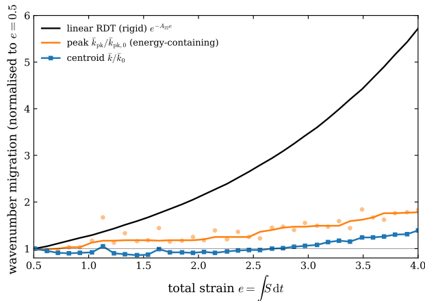
Figure 8. Migration of the spectral peak (energy-containing wavenumber, orange; points are per-dump values, line a rolling median) and the centroid (blue) along the strained trajectory at the operating point, each normalised to e = 0.5 , against the linear rapid-distortion rigid-translation prediction e^{-A_{22}e} (black). Both the peak and the centroid remain far below the rigid line—the peak migrates only weakly (to less than 2 against a predicted 5.7 at e = 4 )—showing that at \chi = O(1) the eddy relaxation holds back the energy-containing scales themselves, not merely the dissipation tail. This corroborates the intermediate-regime reading of Figure 7 independently of how the dissipation is estimated.
