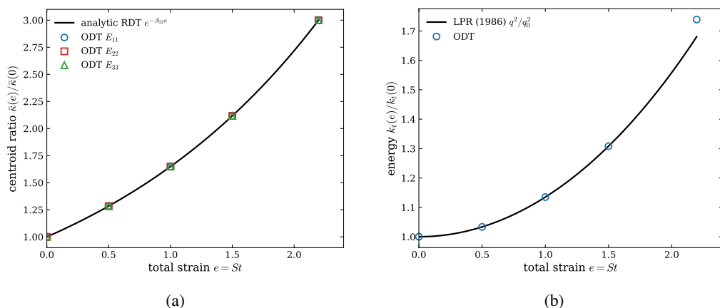
Figure 10. Rapid-distortion limit, with eddy events suppressed and inviscid evolution, against the analytic reference of Lee et al. (1986) used by Chen et al. (2006). (a) Component spectral-centroid migration follows the rigid-translation prediction e^{-A_{22}e} , shown by the solid line, reaching the deformation ratio D = 3 at the end of the straining phase, with the three components coincident. (b) Turbulent kinetic energy follows the plane-strain amplification q^2/q_0^2 , shown by the solid line, reaching 1.74 at e = 2.20 .
