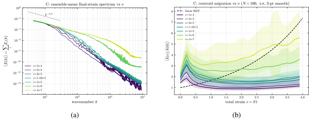
Figure 6. Reynolds-number dependence of the full model (ensemble means, N = 100 per \nu , \pm\sigma ; centroid curves lightly smoothed), for \nu = 10^{-4} , 5 \times 10^{-5} , 2 \times 10^{-5} , 1.42 \times 10^{-5} , 10^{-5} , 10^{-6} , 10^{-7} . (a) Final-strain spectrum E(k) = \sum_i E_i(k) ; the cascade extends further toward high k as \nu falls. The dotted line marks a k^{-5/3} slope for reference. At the two smallest \nu the spectrum flattens into a grid-scale shelf at the cutoff (under-resolved). (b) Centroid migration per \nu against the linear-RDT line (dashed). The resolved cases ( \nu \gtrsim 10^{-5} ) lie below the line; the two lowest- \nu cases exceed it but carry the widest \sigma bands, reflecting the under-resolved grid-scale energy in (a).
