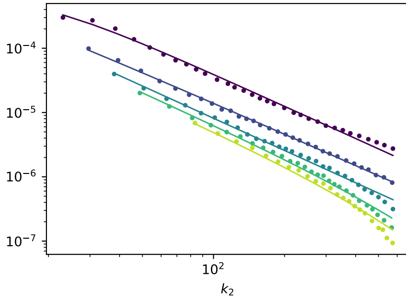
E_{\perp}(k_2) , median + fit
