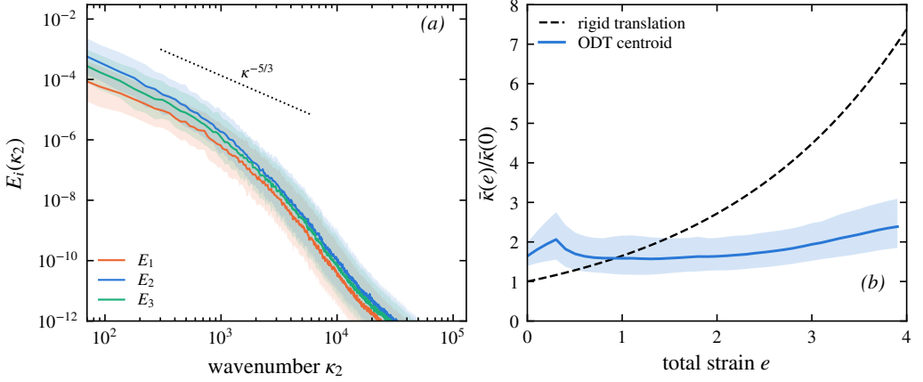
Figure 9. The physical operating point ( \nu \approx 3 \times 10^{-6} , Re_L \approx 4.4 \times 10^3 , 16000 cells; ensemble over 200 realisations, geometric \pm\sigma ). (a) Final-strain component spectra: smooth rolloff with no grid-scale shelf; the upwash E_2 amplified above the streamwise E_1 ; dotted reference slope \kappa^{-5/3} . (b) Total-spectrum centroid migration against the rigid-translation law (dashed): the broadband distortion that linear theory cannot represent, at the operating point and with the noise averaged out.
