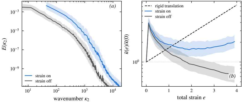
Figure 8. Full model against the matched no-strain baseline at \nu = 10^{-5} (ensemble means over 128 realisations, geometric \pm\sigma bands). (a) Final-strain total spectrum E(\kappa_2) : the full model (strain on) extends to higher wavenumber than the baseline (strain off) but remains broadband, not a rigid translation. (b) Centroid migration: the baseline relaxes below unity, the full model is lifted above it by the compression, yet stays far below the rigid-translation line (dashed). The gap between the two solid curves is the distortion attributable to the mean strain at this Reynolds number.
