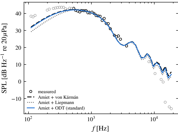
Bampanis 2022 (ECL), flat plate, U=27 m/s
