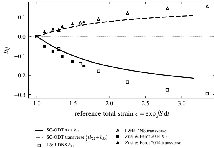
Figure 5. Reynolds-stress anisotropy under axisymmetric contraction: SC-ODT (lines; ensemble mean over 1000 realisations) against the DNS of Lee & Reynolds (1985) (open markers) and the independent DNS of Zusi & Perot (2014) (filled markers, their highest rate, over c \leq 1.65 ). Solid/ \square : the compressed axial component b_{11} ; dashed/ \triangle : the transverse component \frac{1}{2}(b_{22} + b_{33}) . The model tracks the sign and monotonic growth of both, and the two DNS agree where they overlap; the magnitude is under-predicted at large strain by the closure gap common to the second-moment family (§ 3.2), not by the line.
