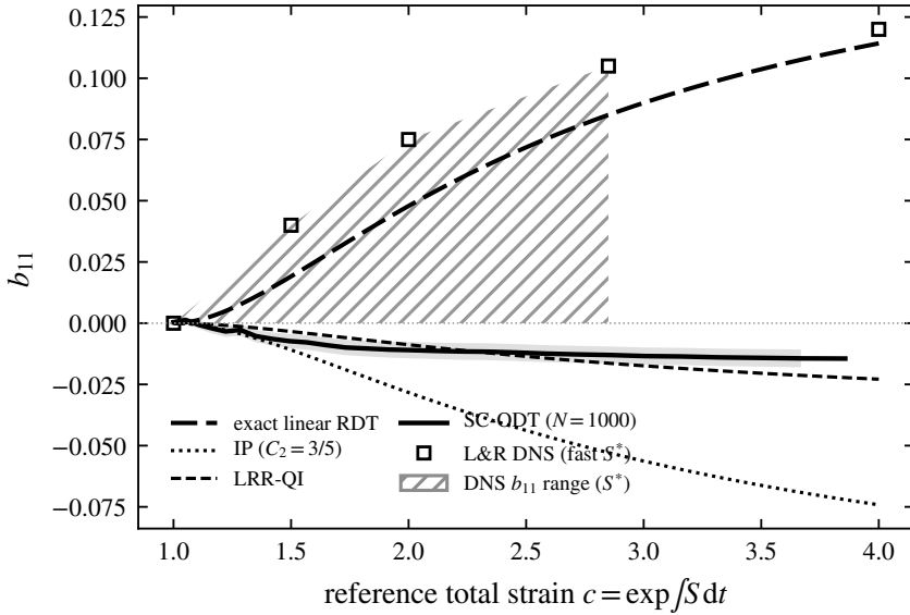
Figure 6. The unstrained-direction anisotropy b_{11} under plane strain: SC-ODT (solid, 1000 realisations) against exact linear rapid distortion (long-dashed, wavevector-ensemble integration), the IP (dotted) and LRR-QI (short-dashed) closures, and the DNS of Lee & Reynolds (1985) (open squares; hatched band = DNS range over slow-to-fast S^* ). The fast-strain DNS tracks exact RDT, whose rapid pressure–strain feeds the neutral direction; the single-point closures—and SC-ODT, built on them—miss this orientation-carried redistribution, the deficiency measured and localised in § 5.6.
