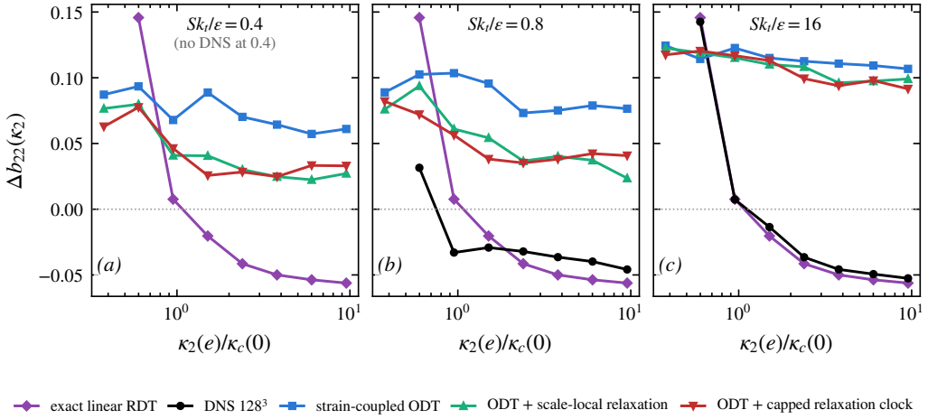
Figure 16. The five-way comparison on the benchmark observable of § 4.6.1: strain-induced upwash anisotropy per wavenumber band at e = 1 , for exact linear RDT, DNS, the strain-coupled model, and the model with each mechanism form (adaptive depth; size-capped relaxation clock), at Sk_t/\varepsilon = 0.4, 0.8 and 16 (ODT: 1024 realisations per case, same binary and precursor protocol; DNS and companions as in § 4.6; no DNS exists at 0.4 , where exact RDT is the reference—at fixed total strain it is independent of the strain rate). At rapid strain the DNS realises the exact-RDT allocation; the mechanism moves the model towards the DNS increasingly as the rapidity falls.
