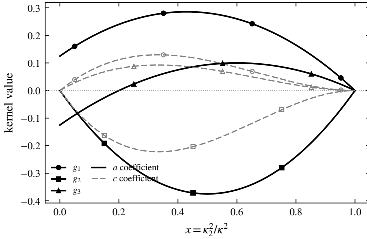
Figure 13. Rapid pressure–strain closure kernels g_1 (circles), g_2 (squares), g_3 (triangles) (eqs. (5.7)–(5.9)) against the angular variable x = \kappa_2^2/\kappa^2 . Solid curves: coefficient of the isotropic-like spectral scalar a ; faint grey dashed curves: coefficient of the anisotropy scalar c . The kernels sum to zero at every x (energy conservation, eq. (5.10)) and vanish at x = 1 . Averaged over an isotropic spectrum they give the ratio +\frac{1}{5} : -\frac{1}{5} : 0 (eq. (5.11)), recovering the isotropisation-of-production form \Pi_{ij}^{(r)} = \frac{4}{3} k_t S_{ij} (Crow 1968) that underlies the moment closure used in § 4.
