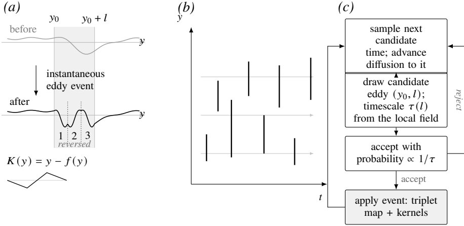
Figure 1. The model at a glance. (a) An eddy event on the sampled interval [y_0, y_0 + l] , taking the field from ‘before’ to ‘after’: the triplet map compresses the profile threefold and inserts three images with the central one reversed (numbered 1–3), and the kernel K(y) = y - f(y) (drawn below) adds c_i K(y) , redistributing kinetic energy among the three velocity components while conserving each component’s momentum and the total energy; the exterior is untouched. (b) The two interleaved mechanisms in the space–time plane: eddy events are instantaneous (vertical bars, at the sampled position y_0 and size l ), arriving as a Poisson sequence whose rate density is set by the instantaneous flow state, while between events the fields advance by deterministic diffusion (faint arrows) and, from § 2.3 onward, the continuous mean-strain forcing. (c) The advancement cycle of the implementation; most sampled candidates are rejected, and the k^{-5/3} cascade is an outcome of repeated sampling from this loop, not an input.
