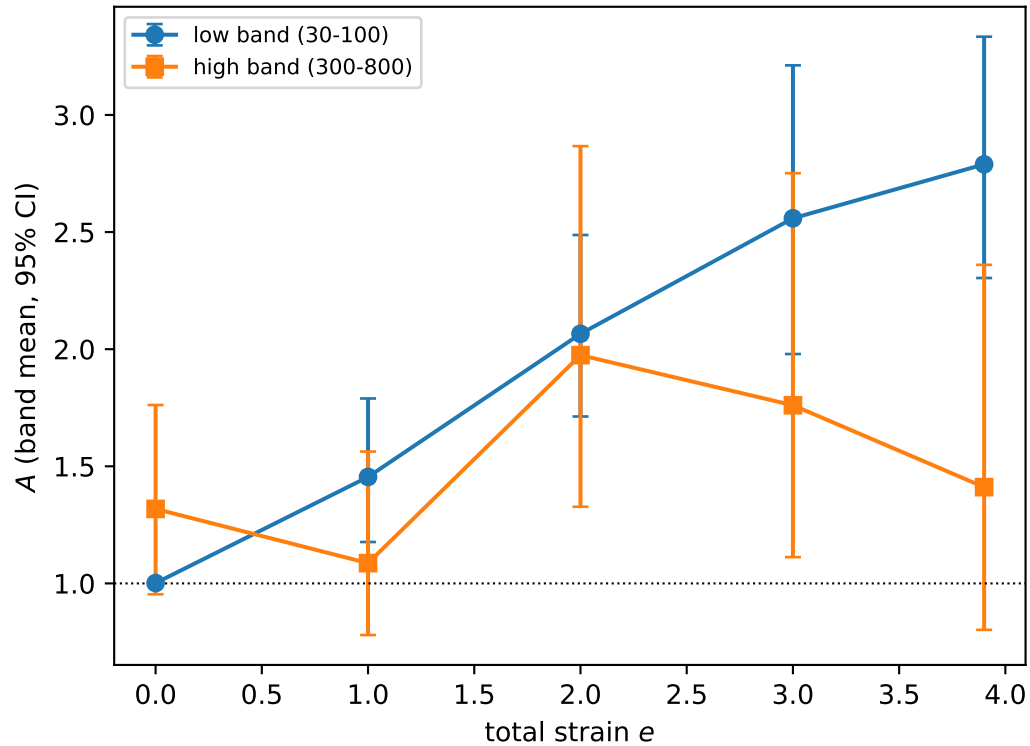
large- vs small-scale anisotropy
