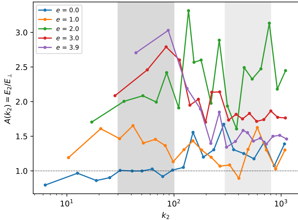
scale-resolved component anisotropy (64 rlz)
