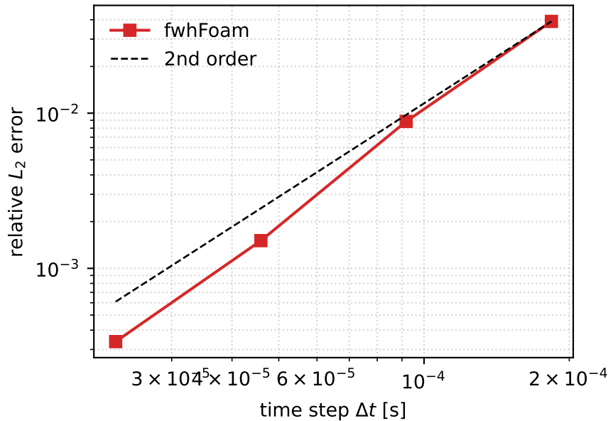
Temporal convergence
