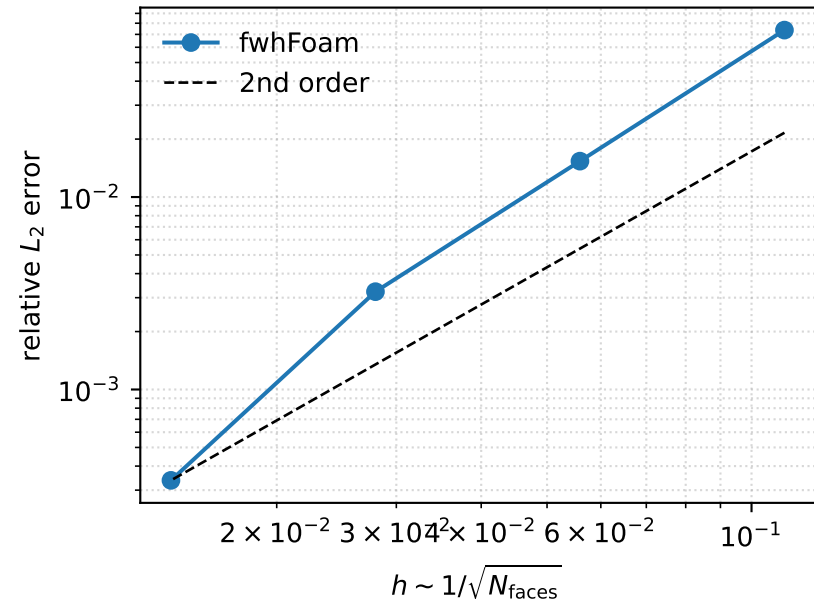
Spatial convergence
